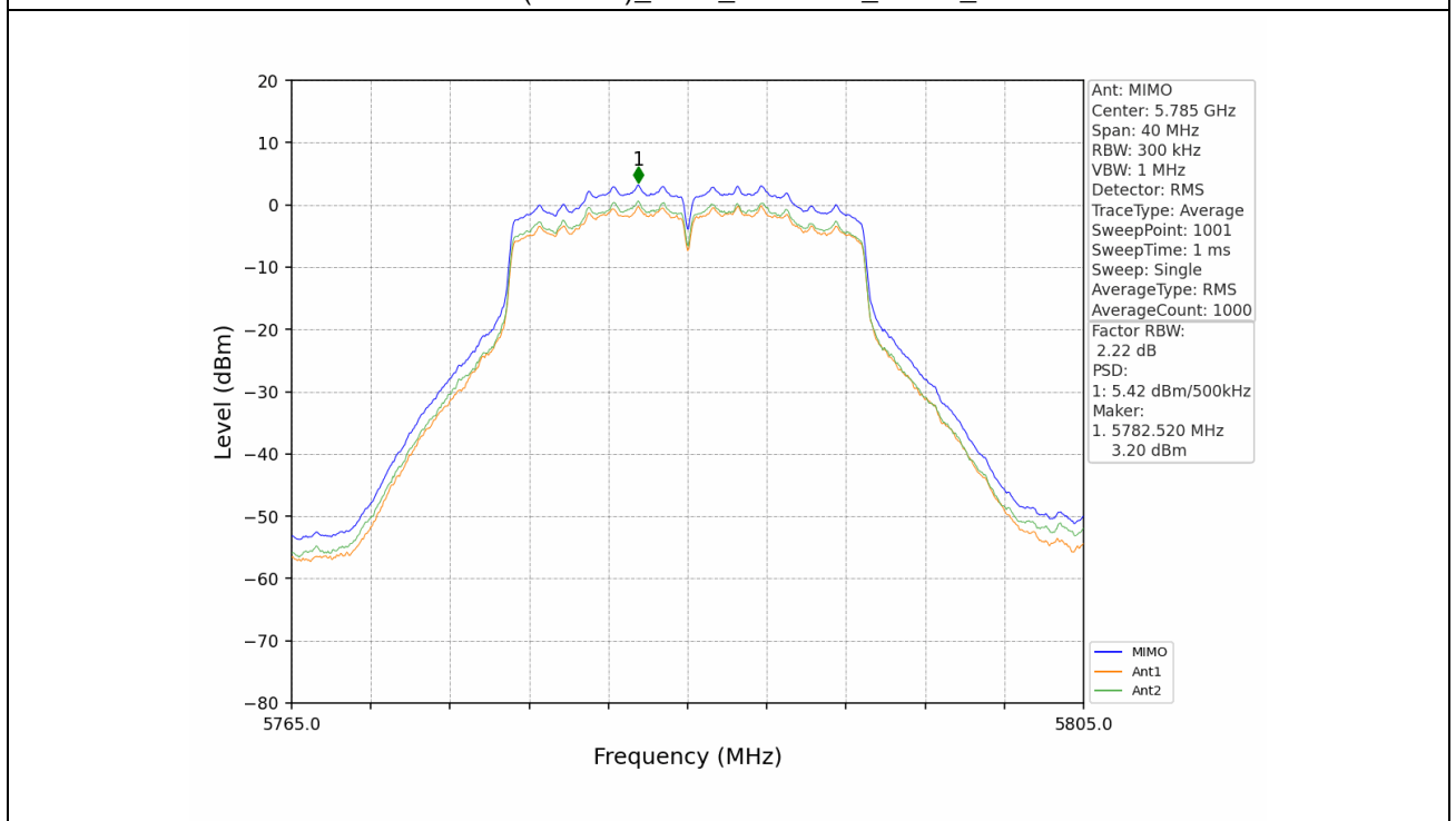
802.11ac(VHT20)_MCH_5785MHz_MIMO_NTNV
