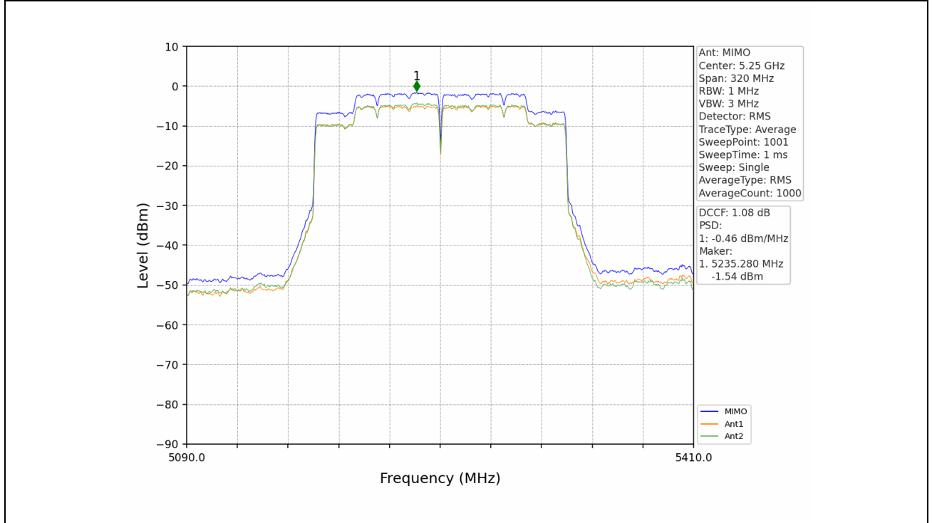
802.11ax(HEW160)_MCH_5250MHz_2xRU996_Left_MIMO_NTNV
