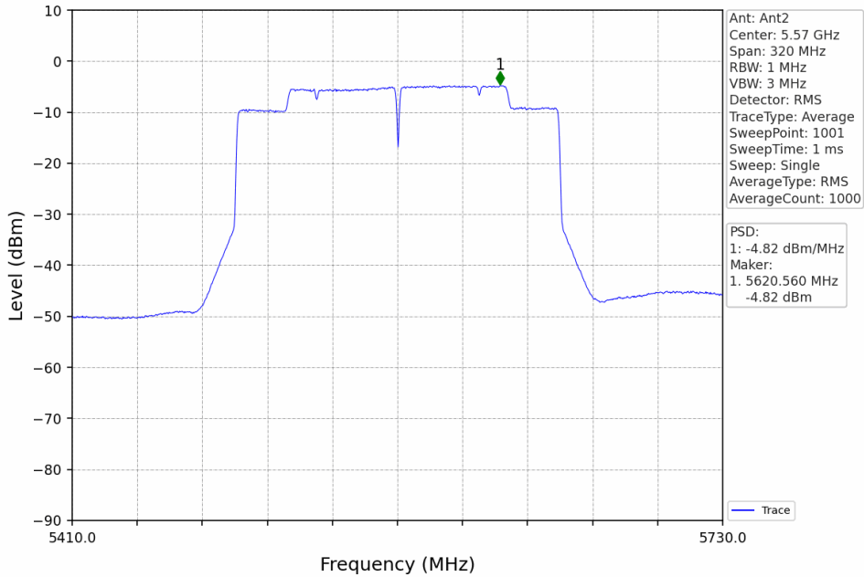
802.11ax(HEW160)_MCH_5570MHz_2xRU996_Left_MIMO_NTNV
