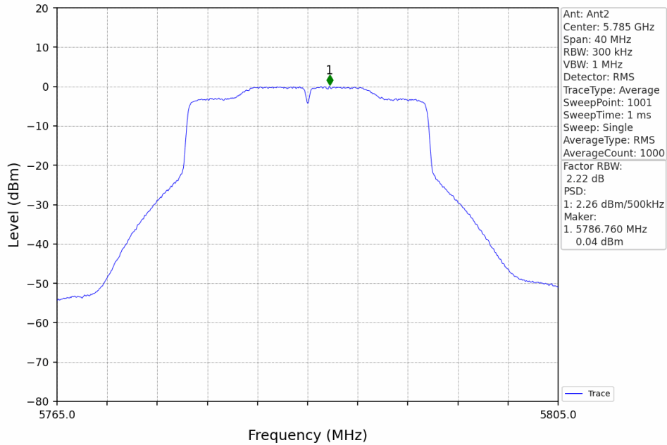
802.11ax(HEW20)_MCH_5785MHz_RU242_Left_MIMO_NTNV
