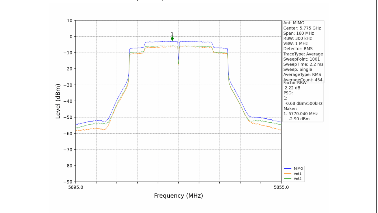
802.11ac(VHT80)_MCH_5775MHz_MIMO_NTNV
