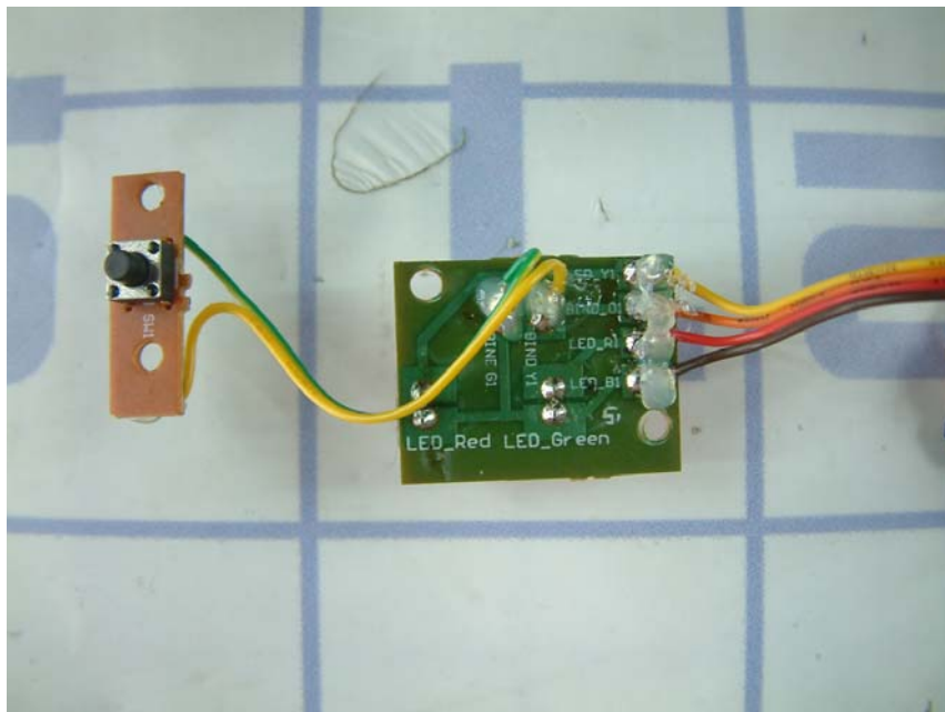
PCB 2 view side 1
