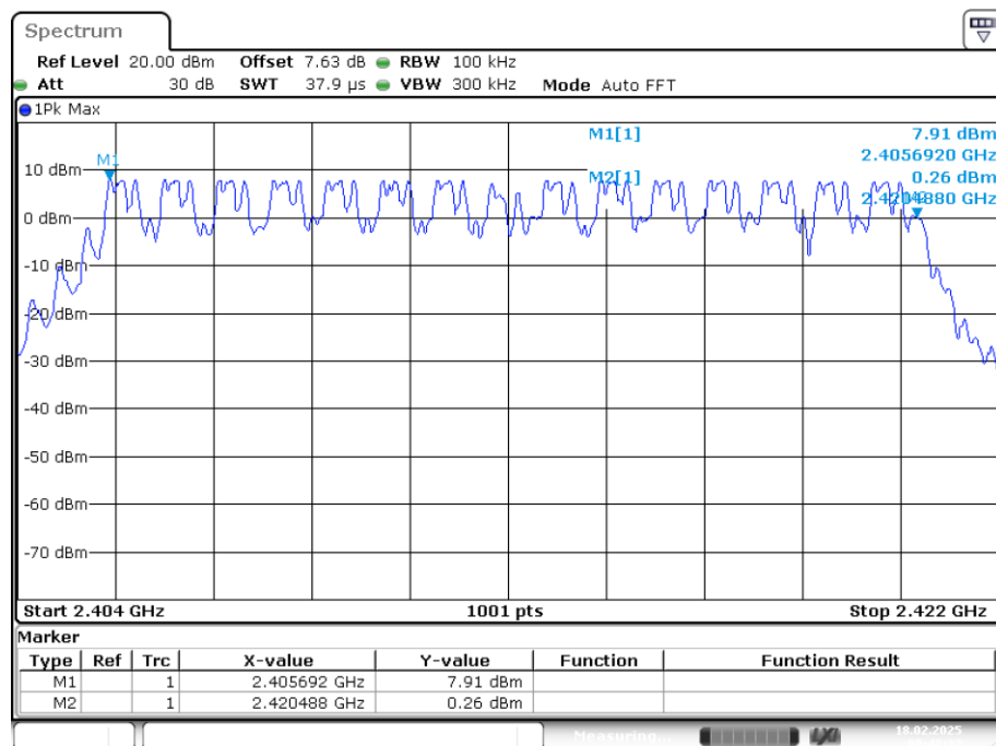
Hopping No. NVNT GFSK 2413MHz Ant1
