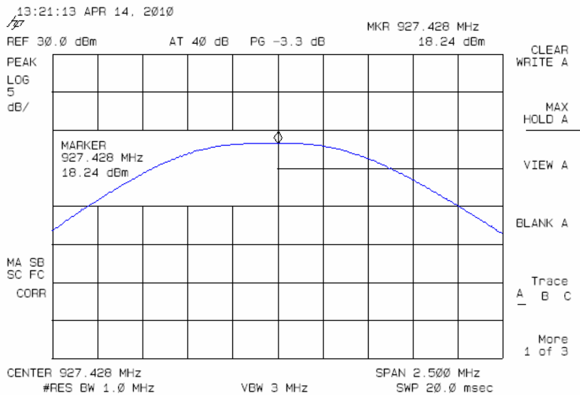
Figure 7 Peak output power high channel
