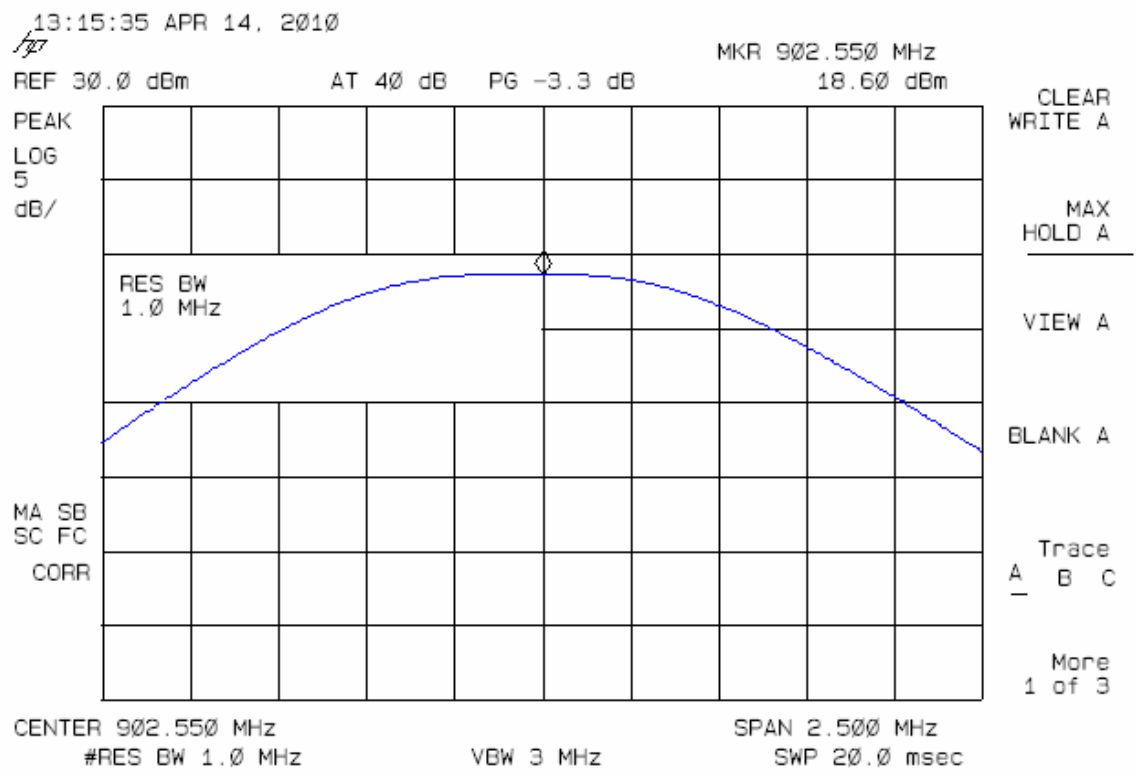
Figure 5 Peak output power low channel.
