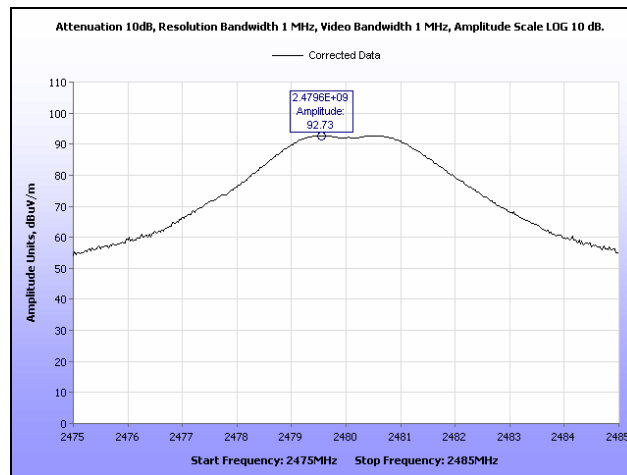
Plot 25. Radiated Restricted Band Edge, Delta Marker, High Channel, Fundamental, Peak
