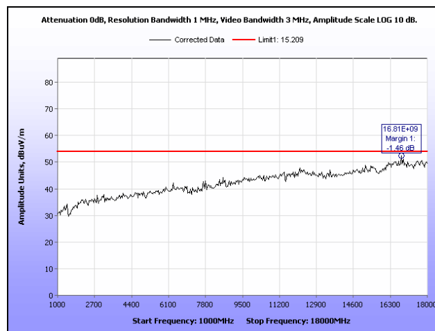
Plot 31. Receiver Spurious Emission, Low Channel, 1 GHz – 18 GHz
