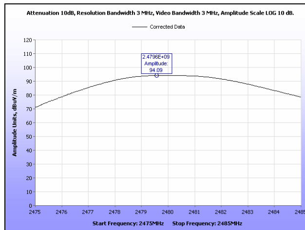
Plot 10. Peak Power Output, High Channel
