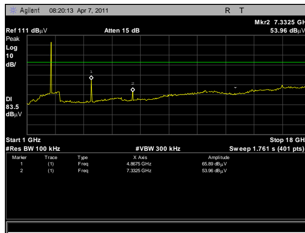
Plot 15. Radiated Spurious Emissions, Mid Channel, 1 GHz – 18 GHz, 20 dBc
