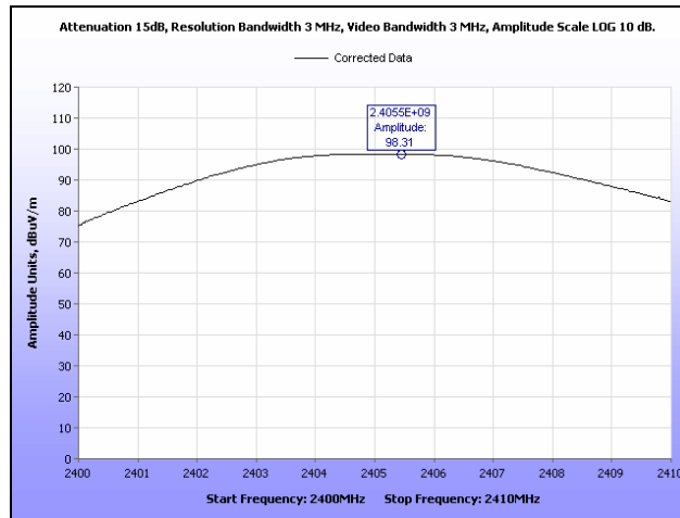
Plot 8. Peak Power Output, Low Channel
