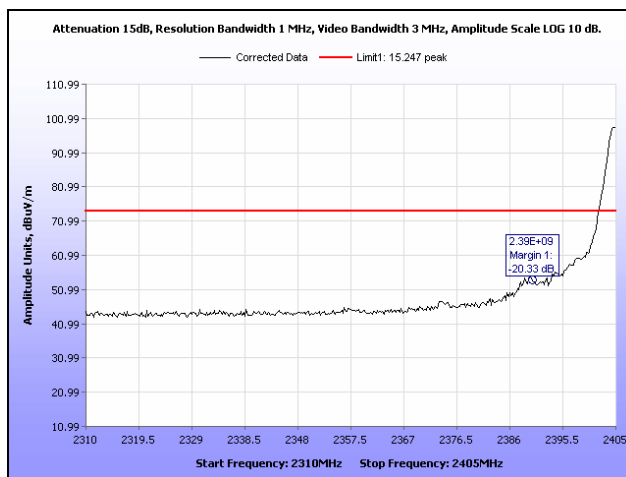
Plot 23. Radiated Restricted Band Edge, Low Channel, Peak
