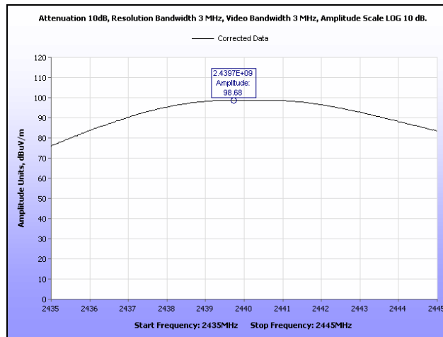
Plot 9. Peak Power Output, Mid Channel
