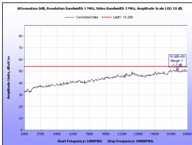
Plot 33. Receiver Spurious Emission, Mid Channel, 1 GHz – 18 GHz
