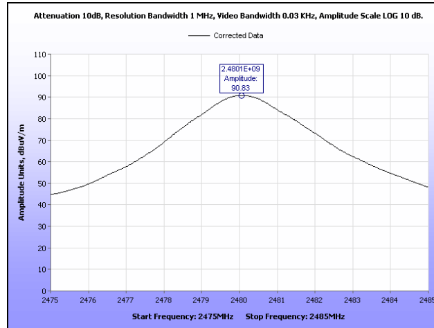
Plot 24. Radiated Restricted Band Edge, Delta Marker, High Channel, Fundamental, Average
