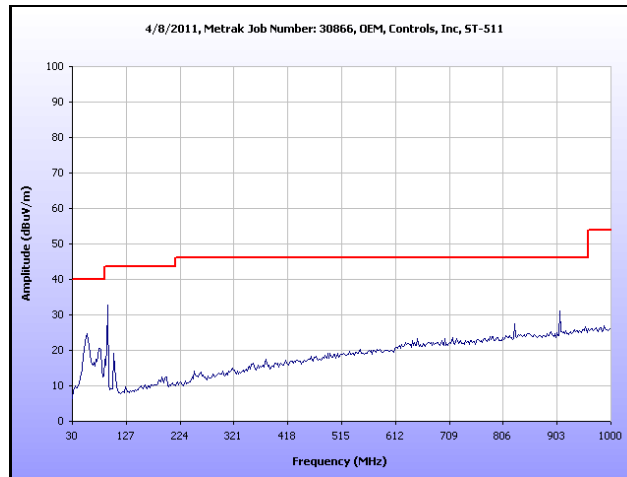
Plot 30. Receiver Spurious Emission, Low Channel, 30 MHz – 1 GHz
