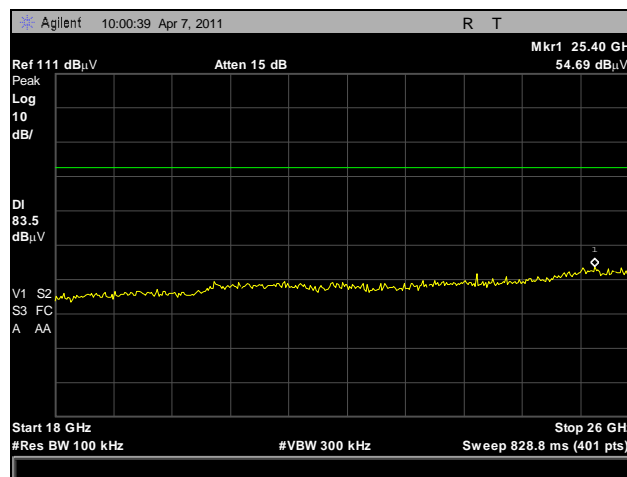
Plot 16. Radiated Spurious Emissions, Mid Channel, 18 GHz – 26 GHz, 20 dBc
