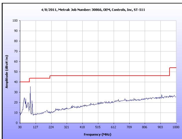
Plot 34. Receiver Spurious Emission, High Channel, 30 MHz – 1 GHz
