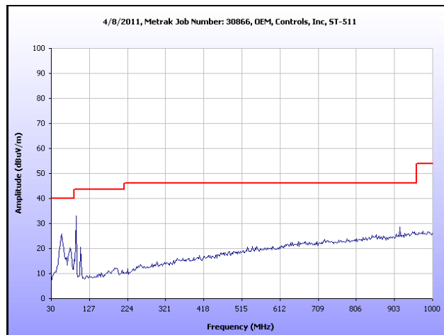
Plot 32. Receiver Spurious Emission, Mid Channel, 30 MHz – 1 GHz
