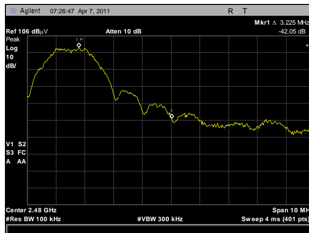
Plot 26. Radiated Restricted Band Edge, Delta Marker, Delta
