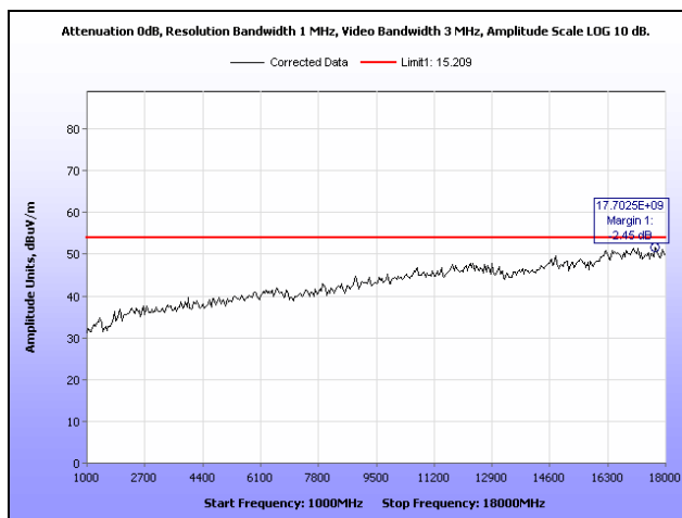
Plot 35. Receiver Spurious Emission, High Channel, 1 GHz – 18 GHz
