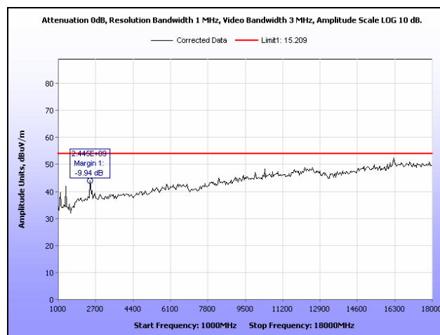
Plot 35. Receiver Spurious Emission, High Channel, 1 GHz – 18 GHz
