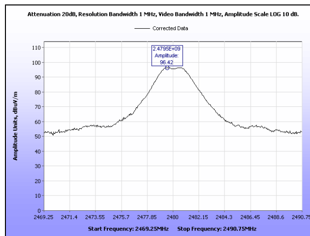
Plot 25. Radiated Restricted Band Edge, Delta Marker, High Channel, Fundamental, Peak
