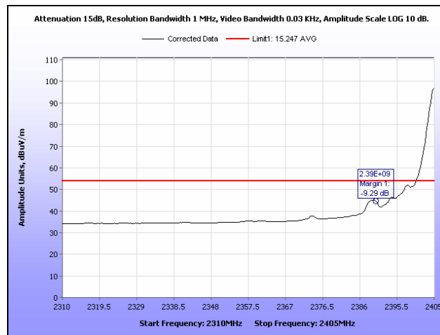
Plot 22. Radiated Restricted Band Edge, Low Channel, Average
