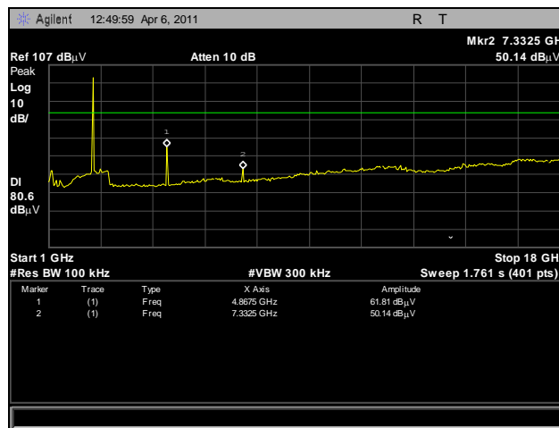
Plot 23. Radiated Spurious Emissions, Mid Channel, 1 GHz – 18 GHz, 20 dBc
