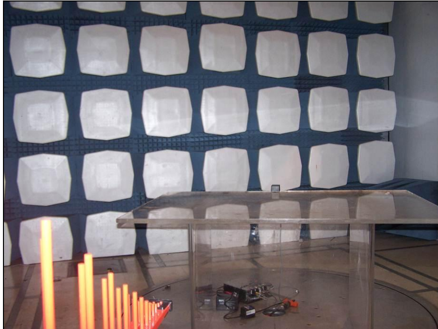
Photograph 5. Radiated Spurious Emissions, Test Setup, Below 1 GHz
