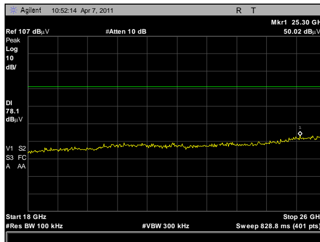
Plot 27. Radiated Spurious Emissions, High Channel, 18 GHz – 26 GHz, dBc
