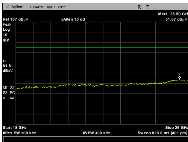
Plot 21. Radiated Spurious Emissions, Low Channel, 18 GHz – 26 GHz, 20 dBc
