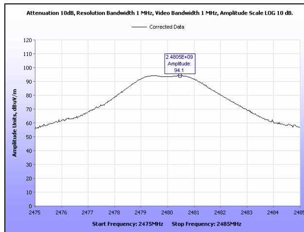
Plot 33. Radiated Restricted Band Edge, Delta Marker, High Channel, Fundamental, Peak
