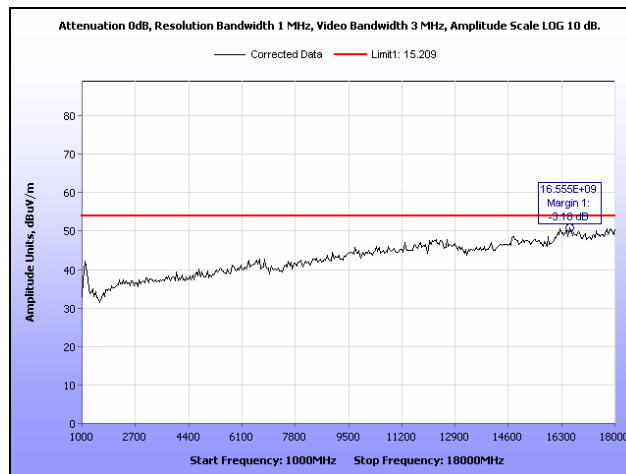
Plot 43. Receiver Spurious Emission, High Channel, 1 GHz – 18 GHz
