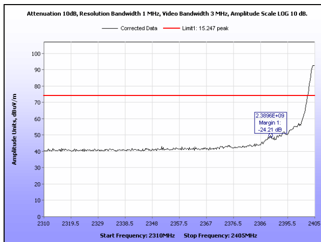
Plot 31. Radiated Restricted Band Edge, Low Channel, Peak
