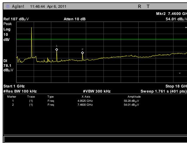
Plot 26. Radiated Spurious Emissions, High Channel, 1 GHz – 18 GHz, 20 dBc
