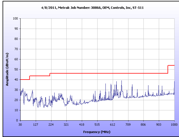
Plot 38. Receiver Spurious Emission, Low Channel, 30 MHz – 1 GHz
