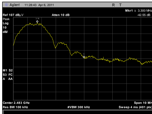
Plot 34. Radiated Restricted Band Edge, Delta Marker, Delta
