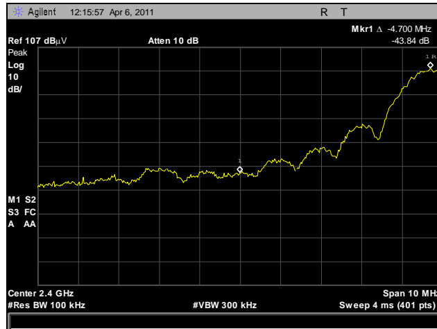
Plot 28. Radiated Spurious Emissions, Low Channel, 20 dBc
