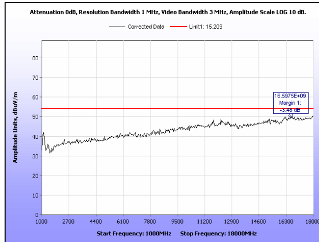
Plot 41. Receiver Spurious Emission, Mid Channel, 1 GHz – 18 GHz
