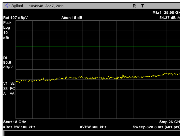
Plot 24. Radiated Spurious Emissions, Mid Channel, 18 GHz – 26 GHz, 20 dBc
