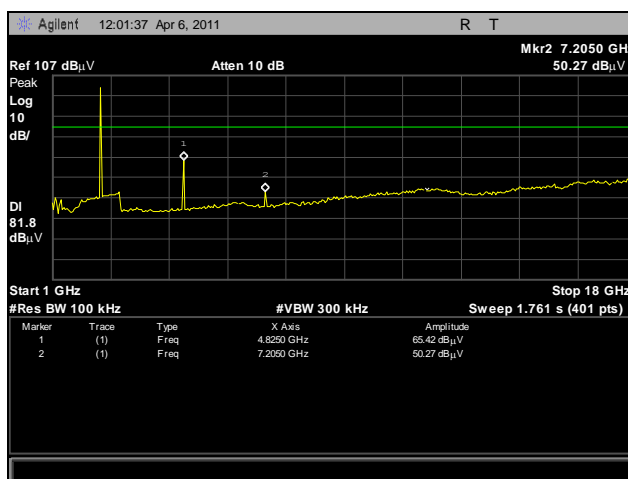
Plot 20. Radiated Spurious Emissions, Low Channel, 1 GHz – 18 GHz, 20 dBc
