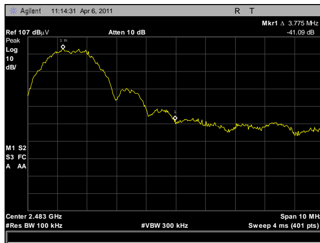
Plot 29. Radiated Spurious Emissions, High Channel, 20 dBc
