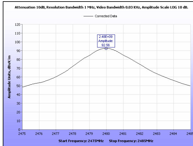
Plot 32. Radiated Restricted Band Edge, Delta Marker, High Channel, Fundamental, Average
