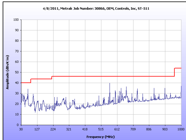
Plot 40. Receiver Spurious Emission, Mid Channel, 30 MHz – 1 GHz
