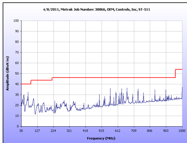
Plot 42. Receiver Spurious Emission, High Channel, 30 MHz – 1 GHz
