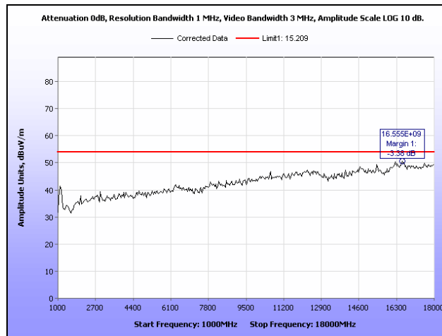
Plot 39. Receiver Spurious Emission, Low Channel, 1 GHz – 18 GHz
