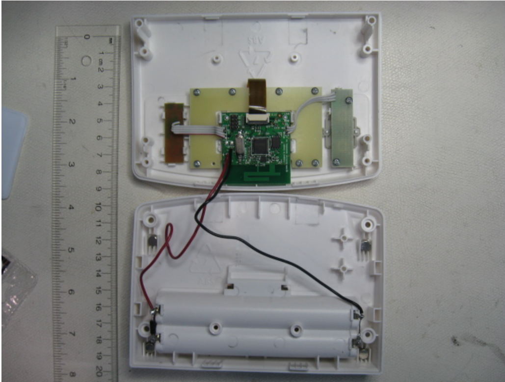
PCB Front
