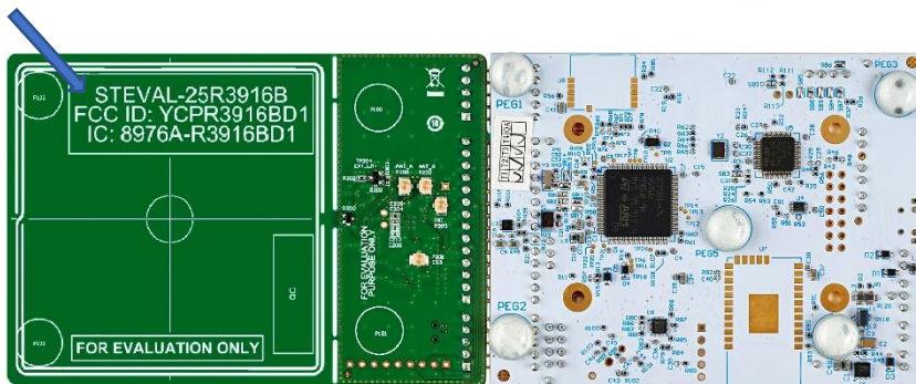
STEVAL-25R3916B Bottom View
