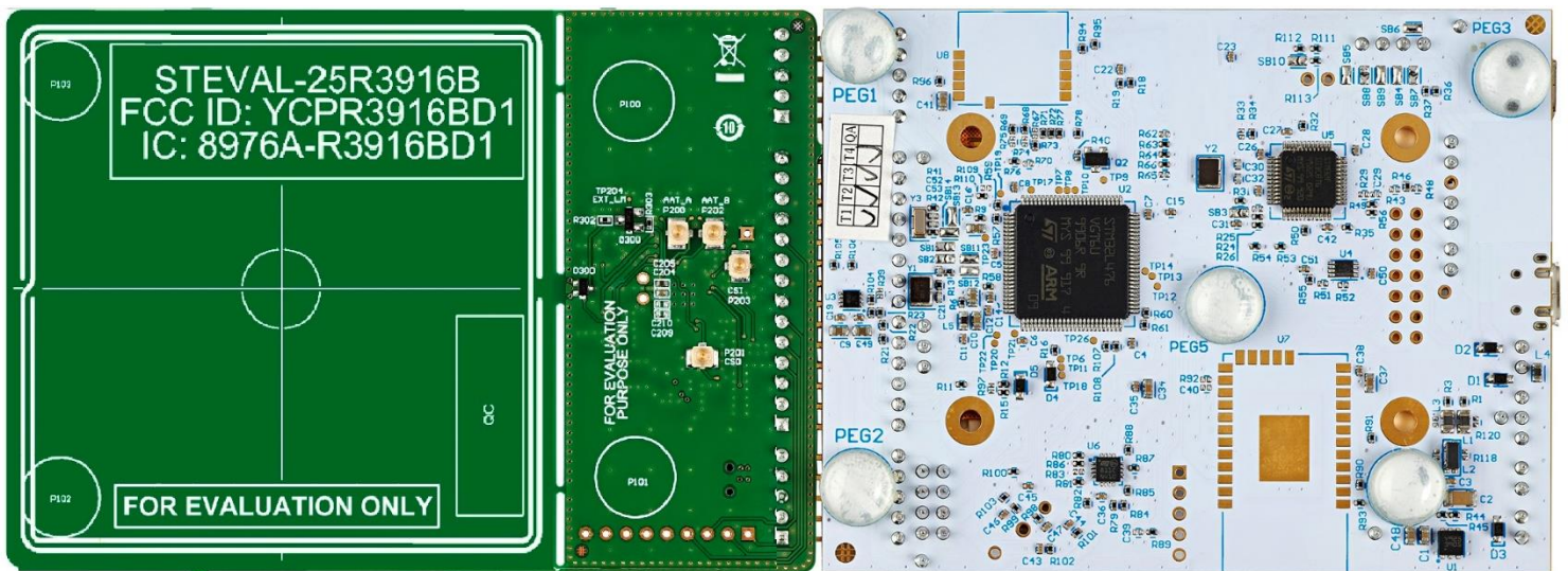
STEVAL-25R3916B Bottom View
