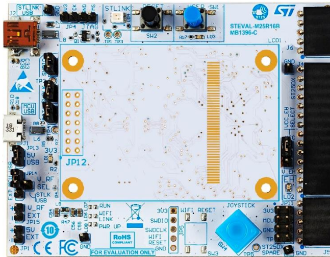
STEVAL-M25R16B Without LCD Top View
