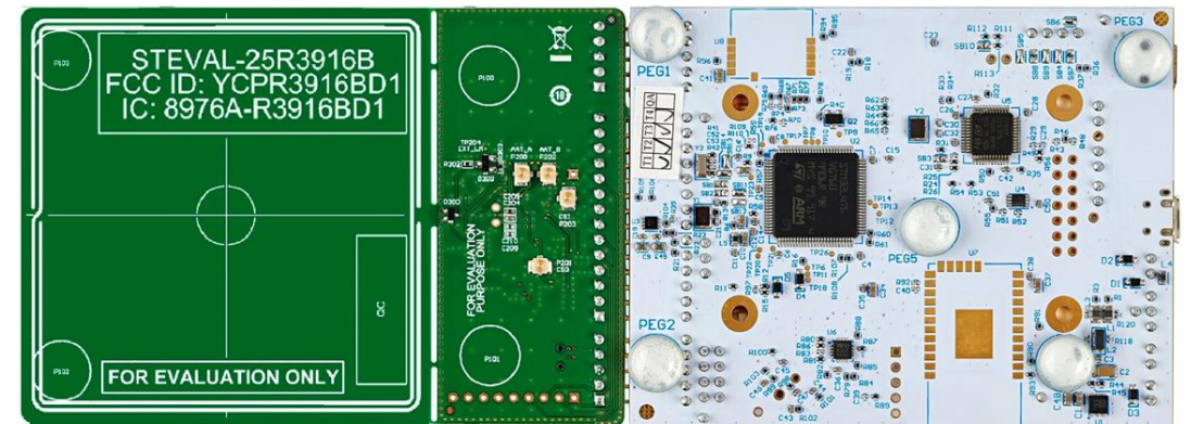
STEVAL-25R3916B Bottom View
