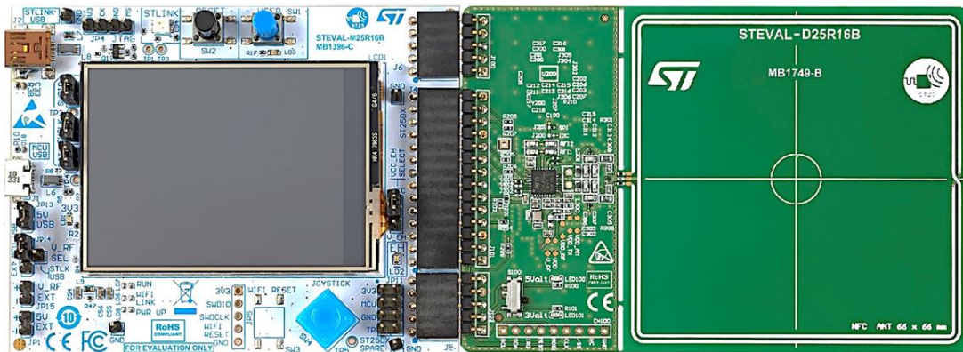
STEVAL-25R3916B Top View
