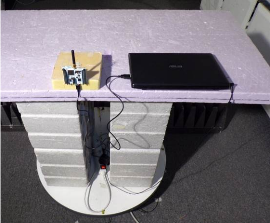
Test setup for frequency below 1GHz
