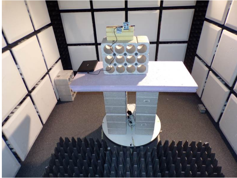
Test setup for frequency above 1GHz
