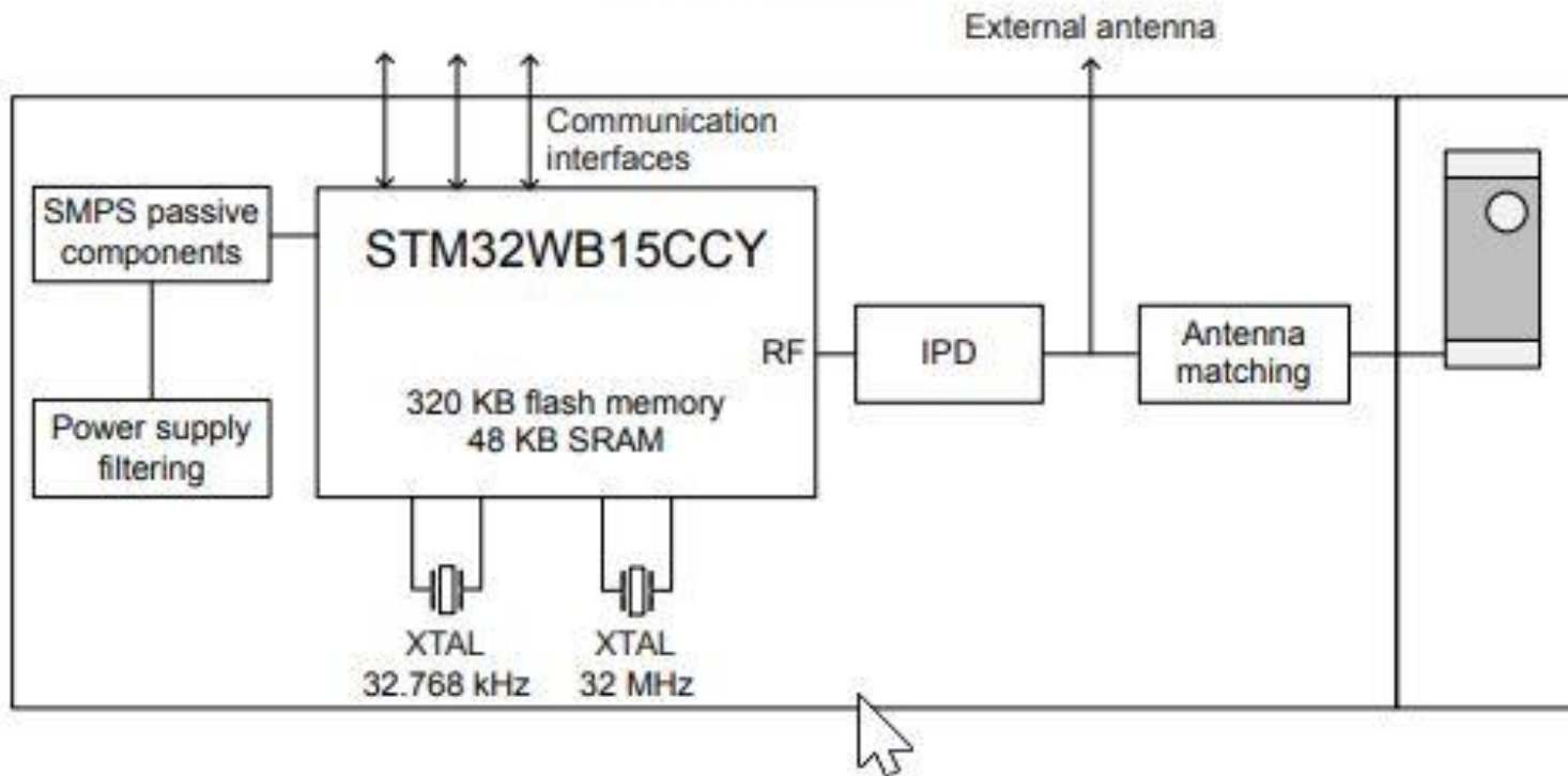
Figure 1. Block diagram
