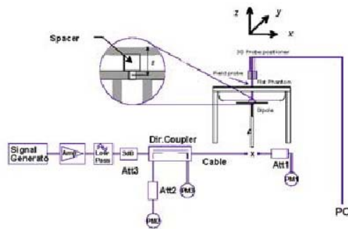
Figure 12.1 Dipole Validation Test Setup
