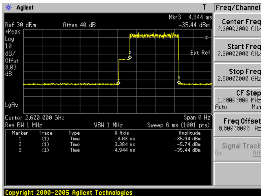
AMC_QPSK 1/2( Plot 2 )
