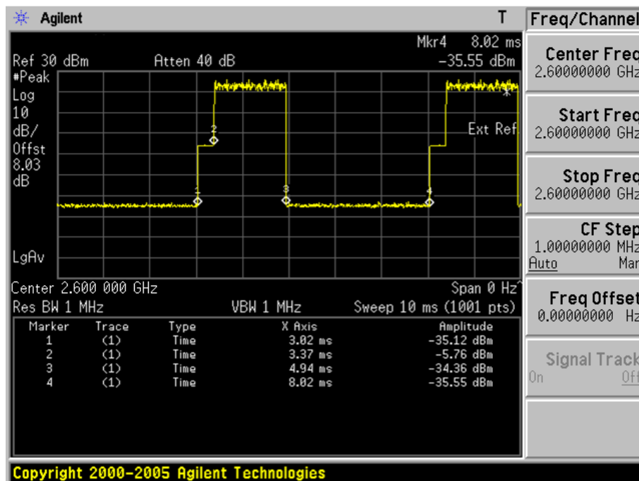
AMC_QPSK 1/2( Plot 1 )
