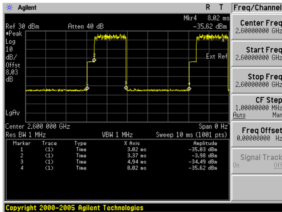
AMC_16QAM 1/2( Plot 2 )
