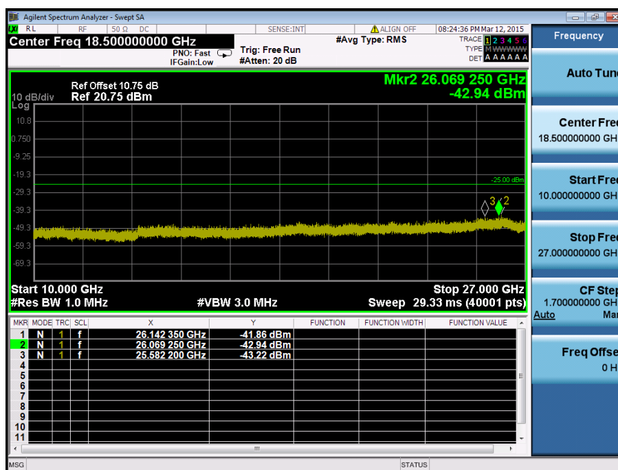
LTE Band 41 / 20MHz / 16QAM - RB Size/Offset (1/99) – Low Channel
