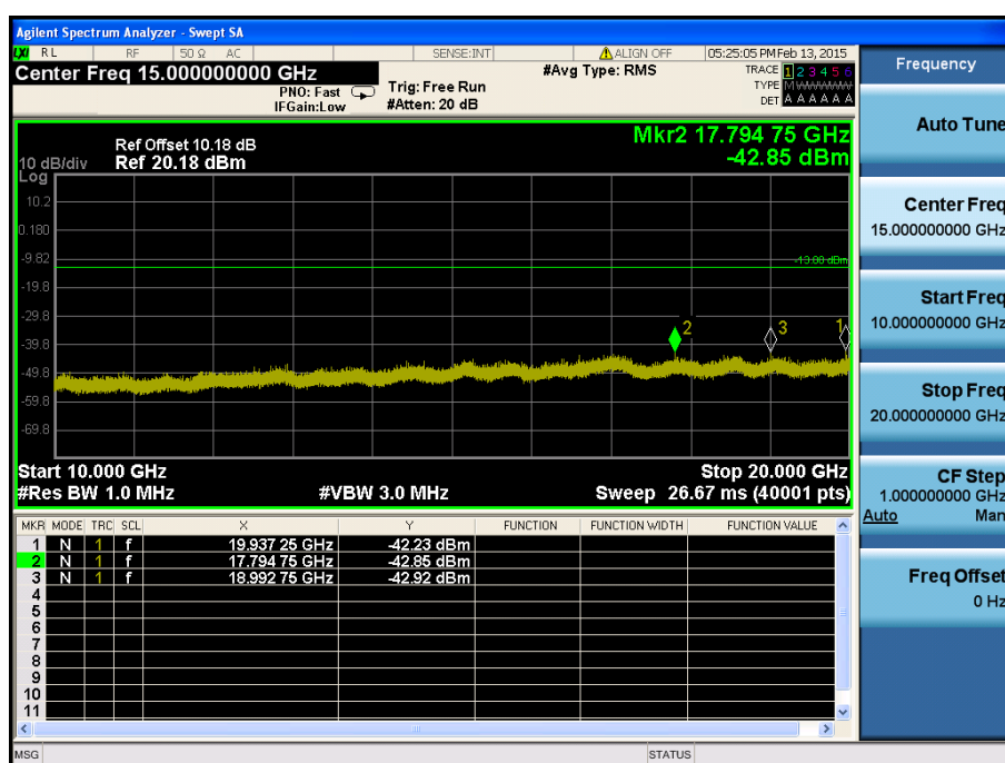
LTE Band 25 / 3MHz / 16QAM - RB Size/Offset (1/0) – Mid Channel
