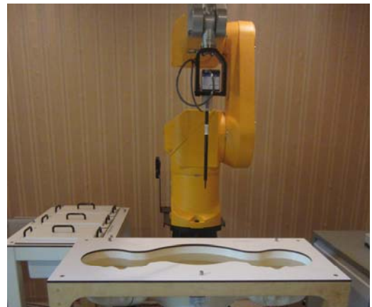
Figure 2.2 DASY4 Test System
