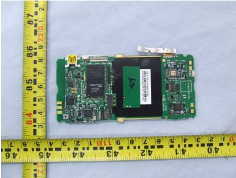
Internal of EUT-9
