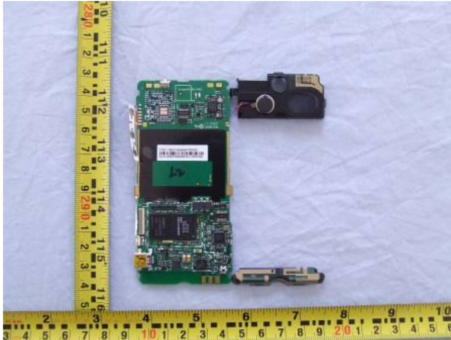
Internal of EUT-7
