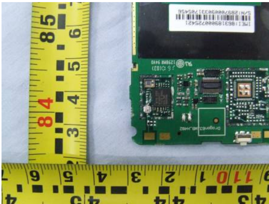
Internal of EUT-10
