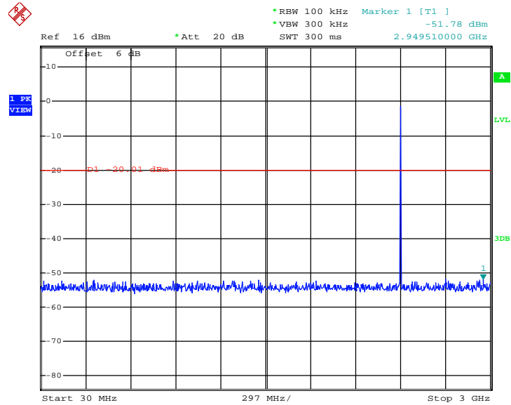
Conducted Spurious Emission Plot on Bluetooth v4.0 LE 1Mbps GFSK Channel 00
