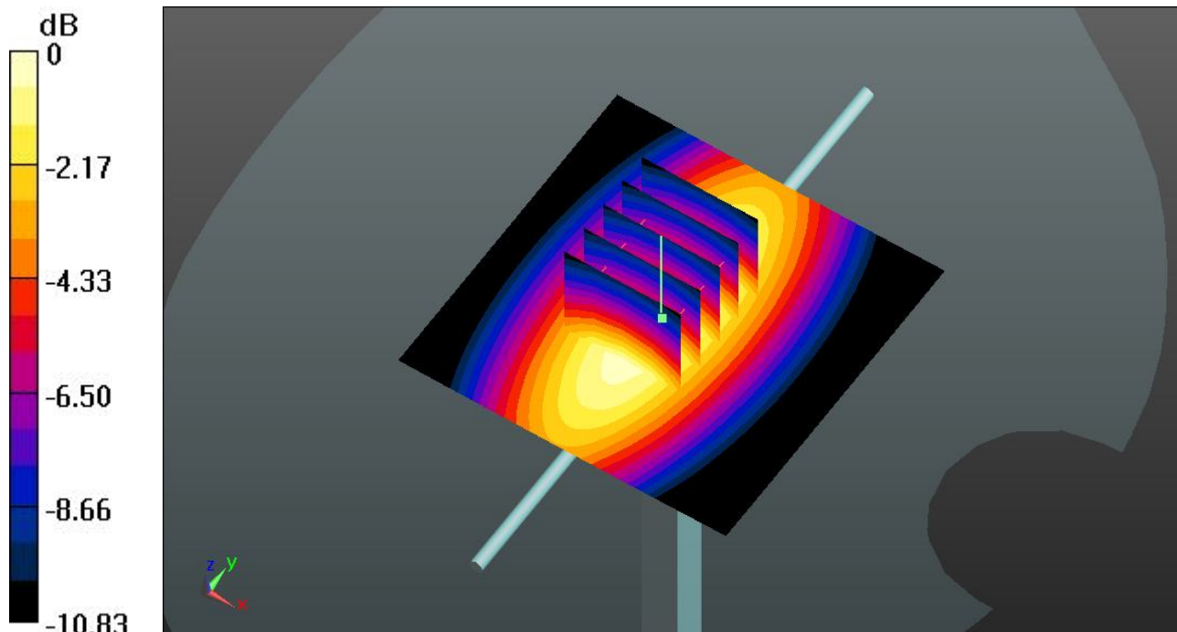
0 dB = 3.19 \text{ W/kg}
