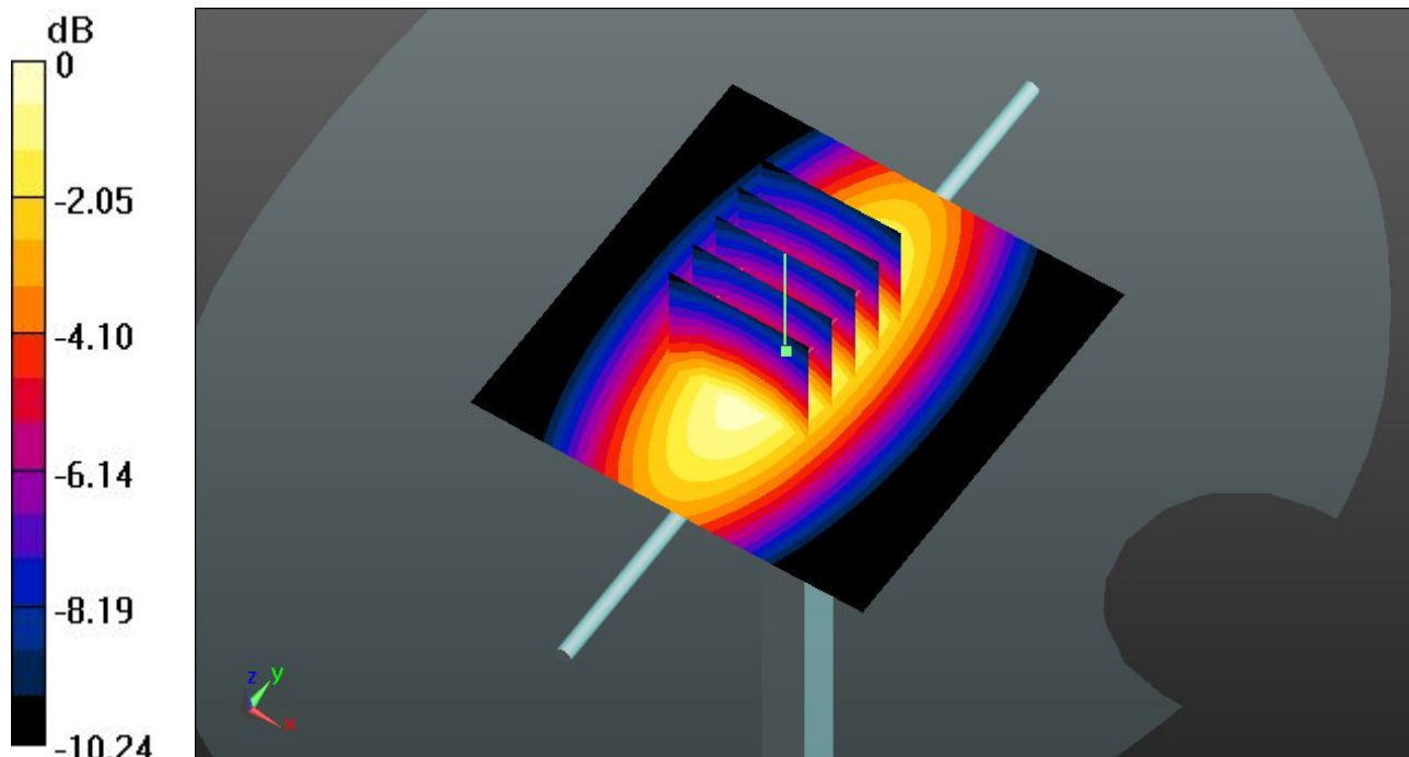
0 dB = 2.63 \text{ W/kg}
