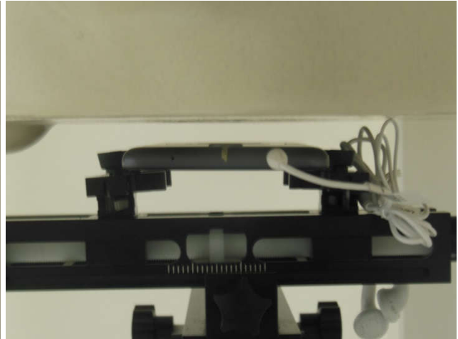
Back with Headset 2, Test Separation 10 mm
