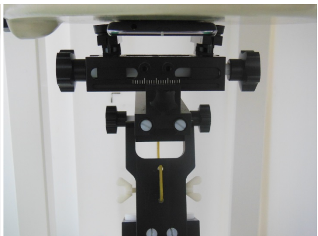
Back, Test Separation 0 cm (Hand SAR)
