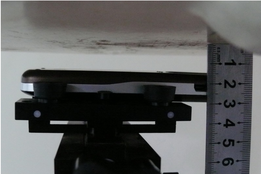
Picture 11: Body, The EUT display towards ground, the distance from handset to the bottom of the Phantom is 15mm
