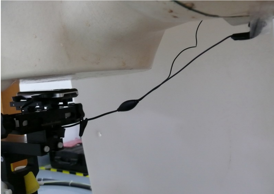
Picture 13: Body with earphone, The EUT display towards phantom, the distance from handset to the bottom of the Phantom is 15mm
