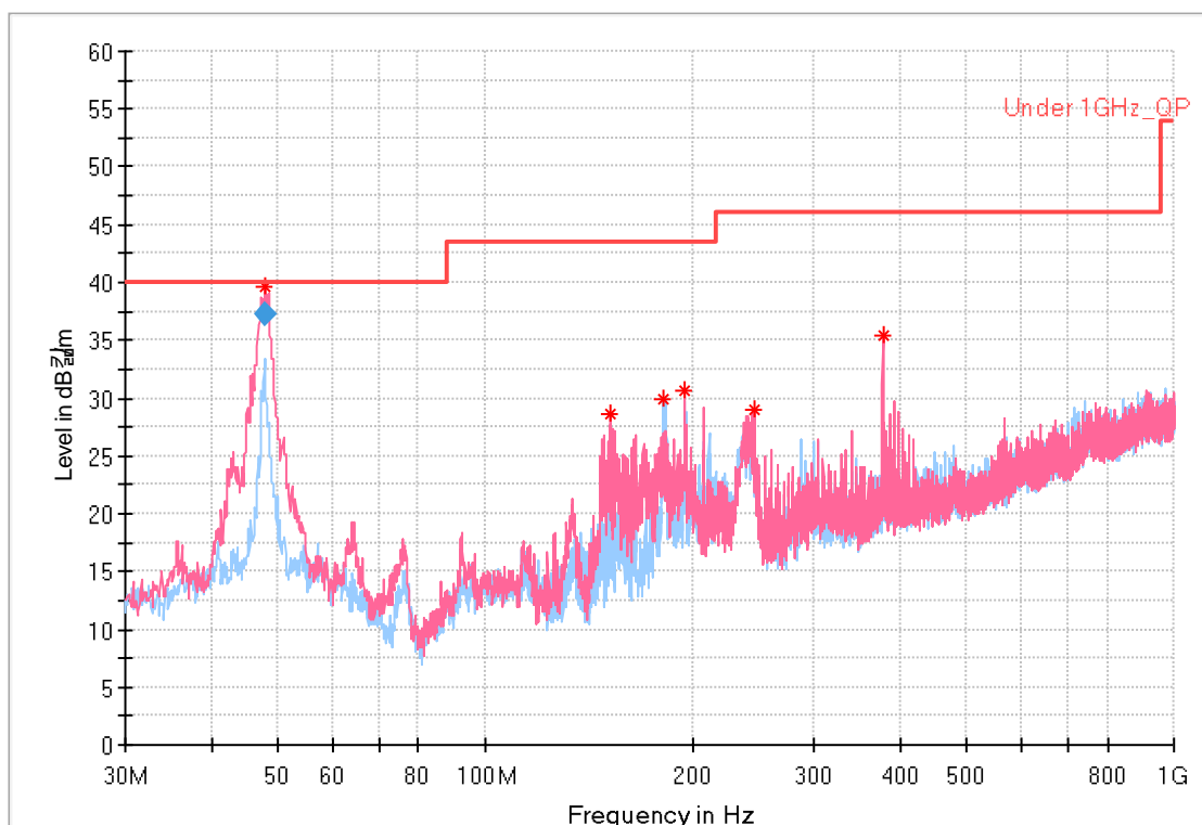
Worst case - RSE(Below 1 GHz)_2DH5 / π/4DQPSK
