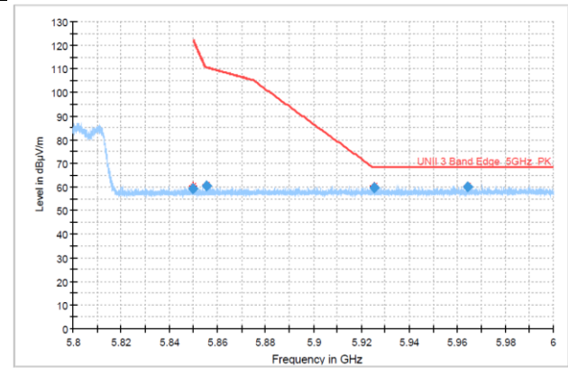
Bandedge_5 775 MHz_High
