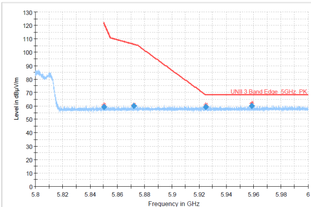
Bandedge_5 775 MHz_High
