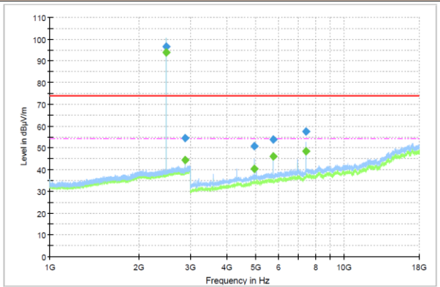
Spurious_Worst case
