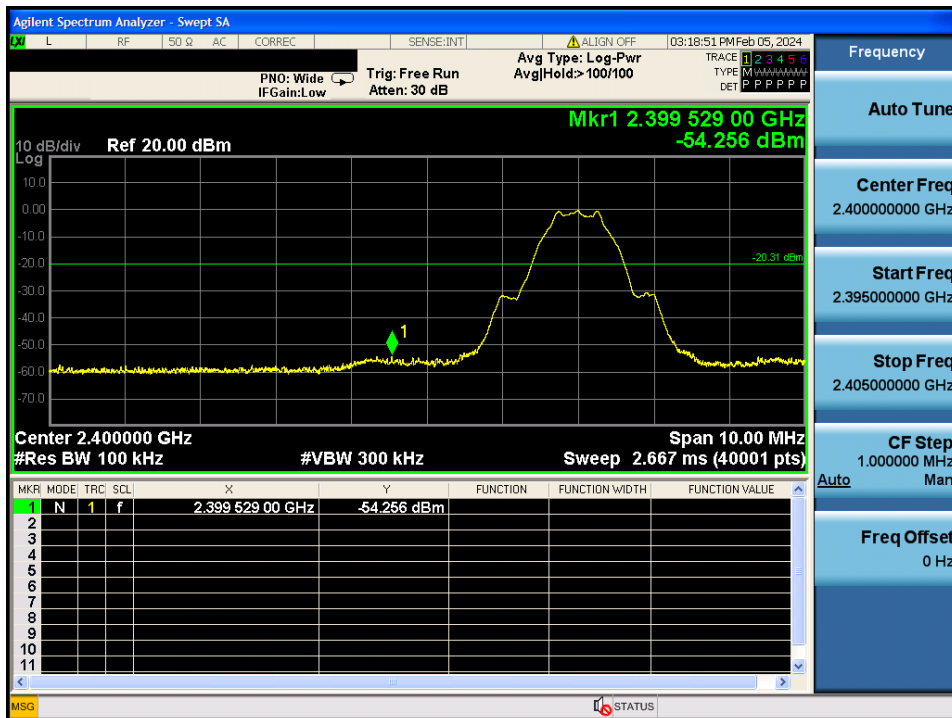
TM 1 Low Band-edge (Test Channel : Lowest)
