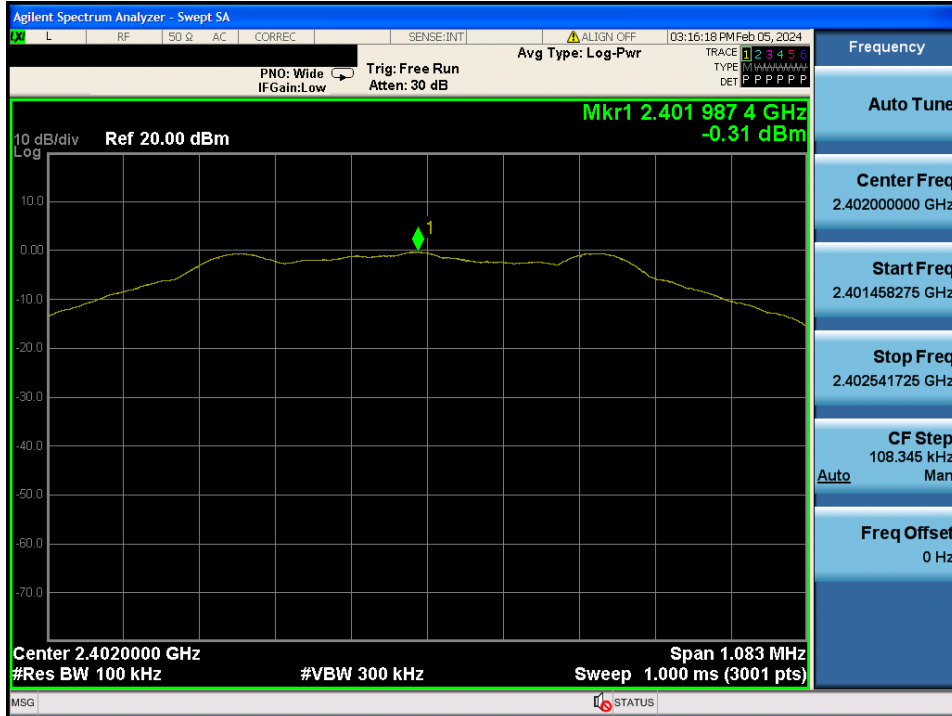
TM 1 Reference (Test Channel : Lowest)
