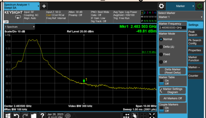
2 480 MHz _ Spurious
