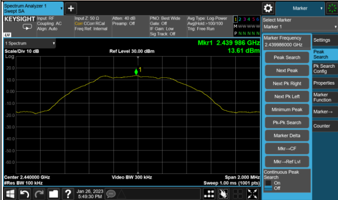
2 440 MHz _ Spurious
