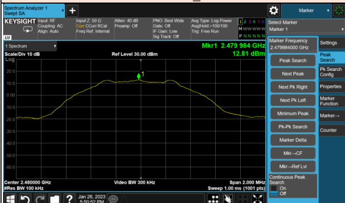
2 480 MHz _ Spurious
