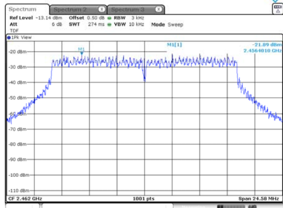
802.11g / 2 462 MHz
