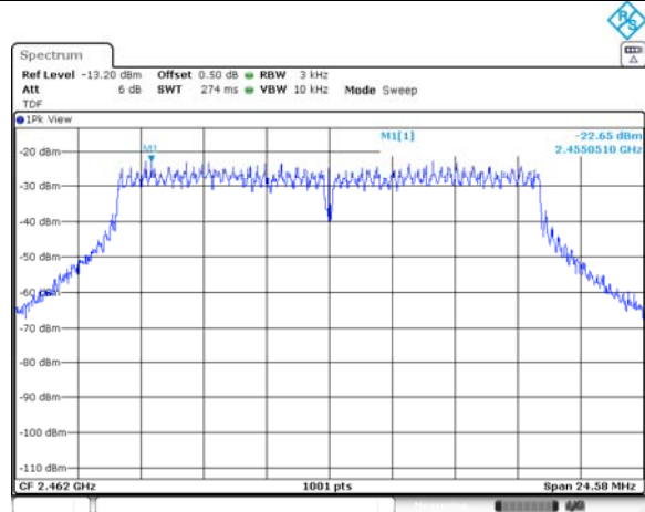
802.11g / 2 462 MHz
