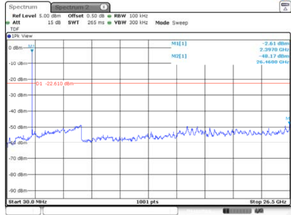
Conducted spurious / 2 441 MHz
