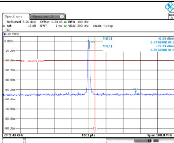
Conducted band-edge / Hopping ch.
