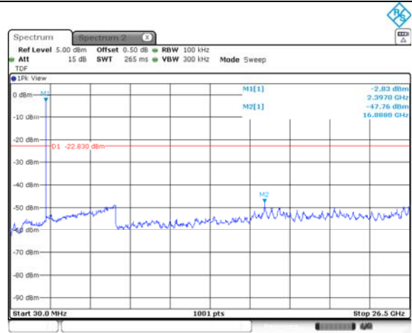
Conducted spurious / 2 441 MHz
