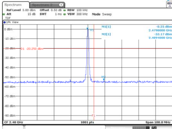
Conducted band-edge / Hopping ch.
