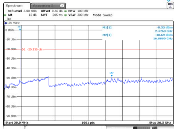
Conducted spurious / 2 480 MHz
