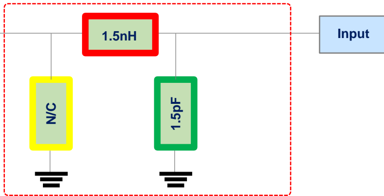
Antenna matching circuit
