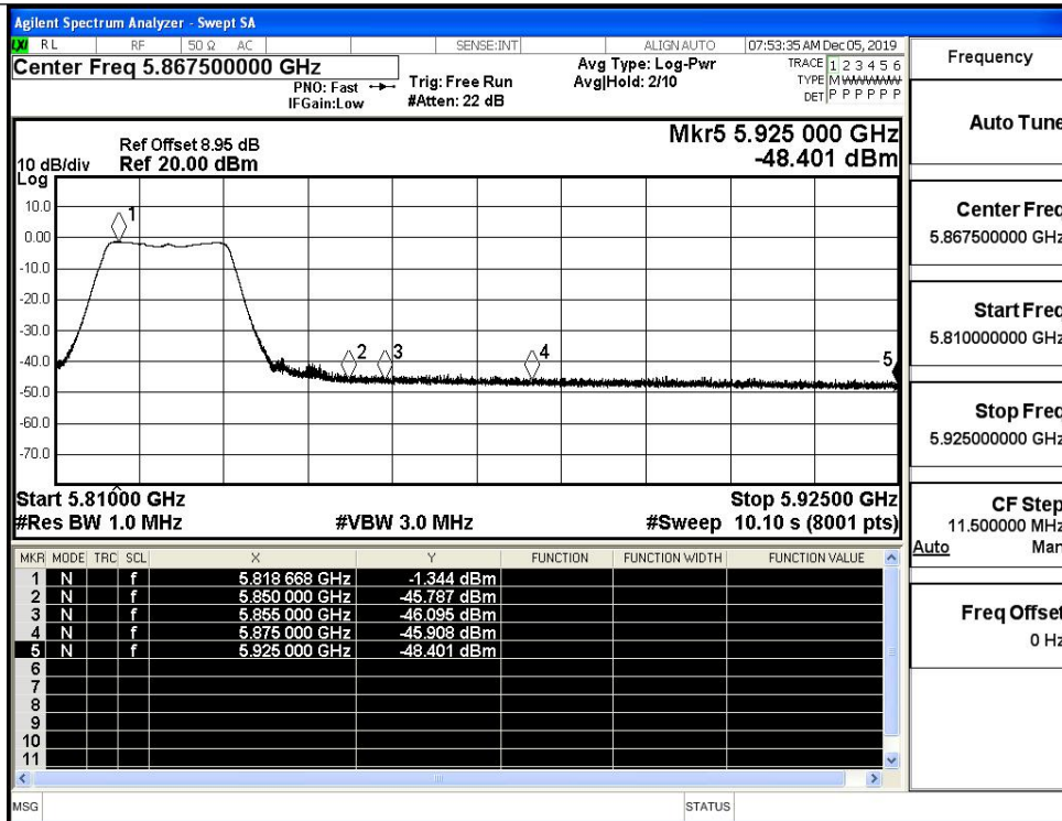
Undesirable Emissions Measurement Undesirable Emissions Measurement (Antenna 1)
