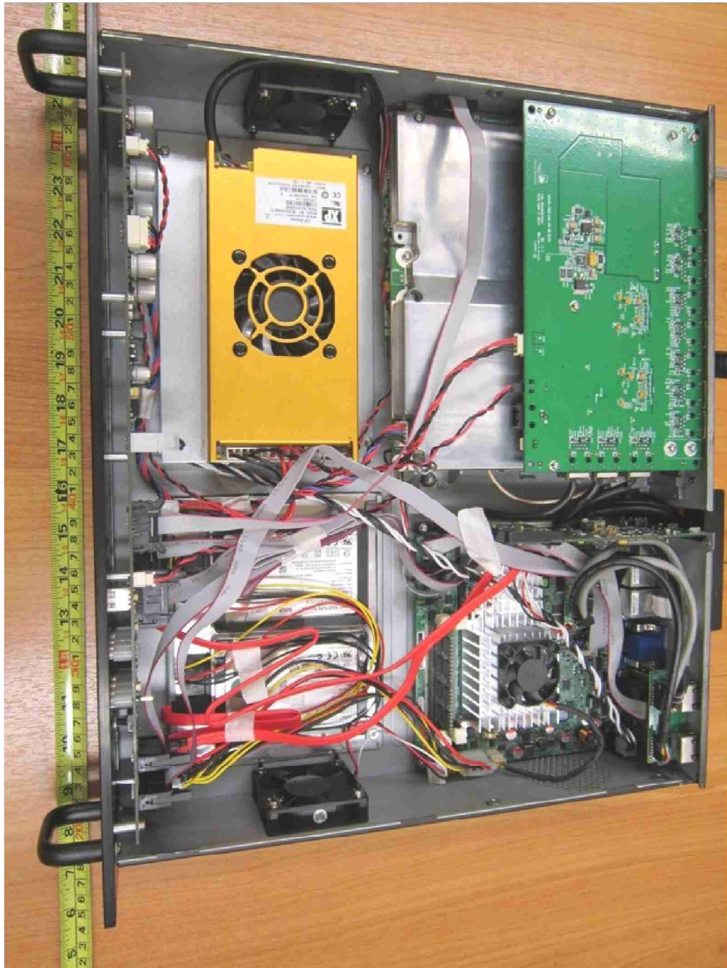
Internal View 1
