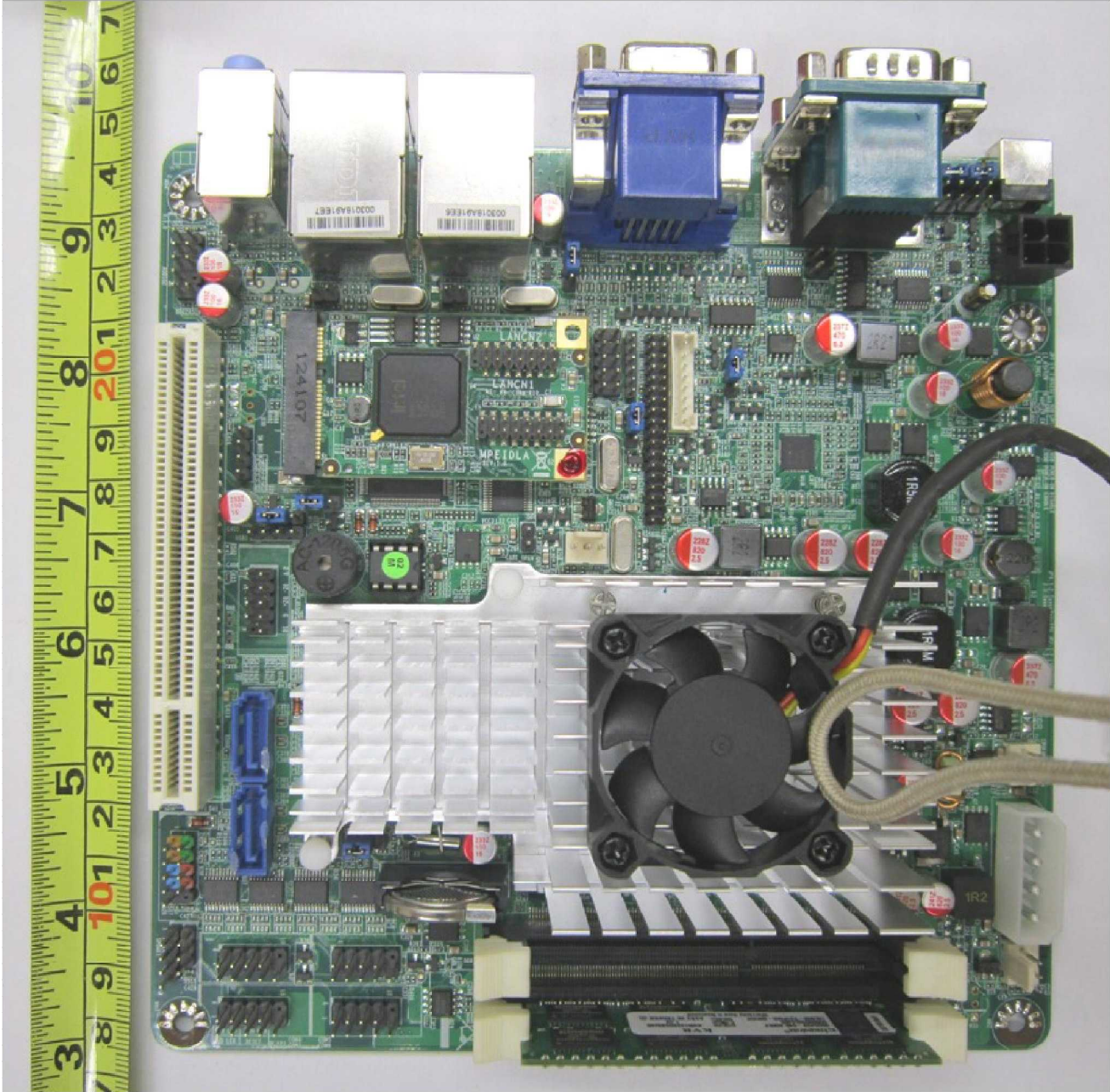
Mother-Board PCB Component Side
