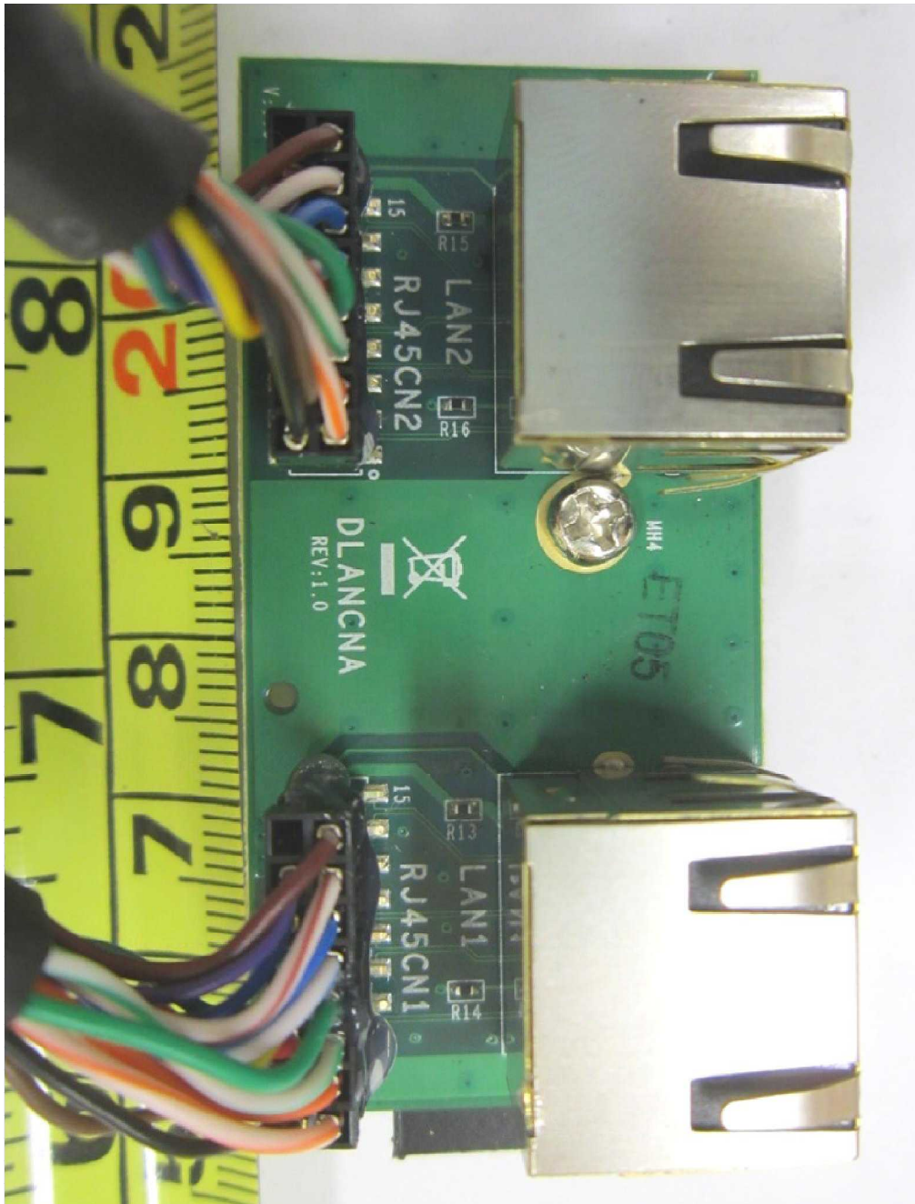
2-LAN Port PCB Component Side
