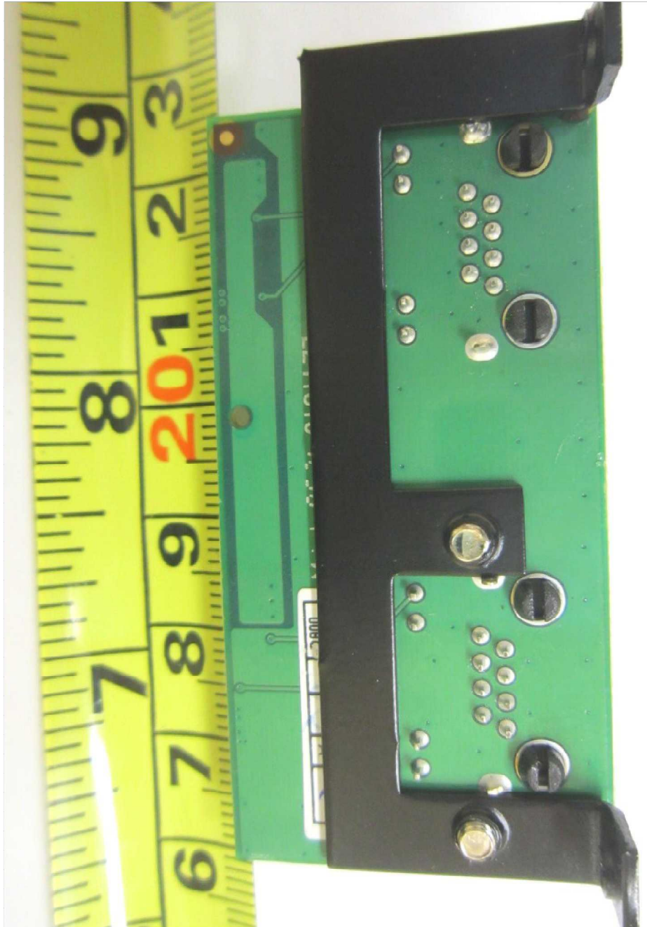
2-LAN Port PCB Trace Side
