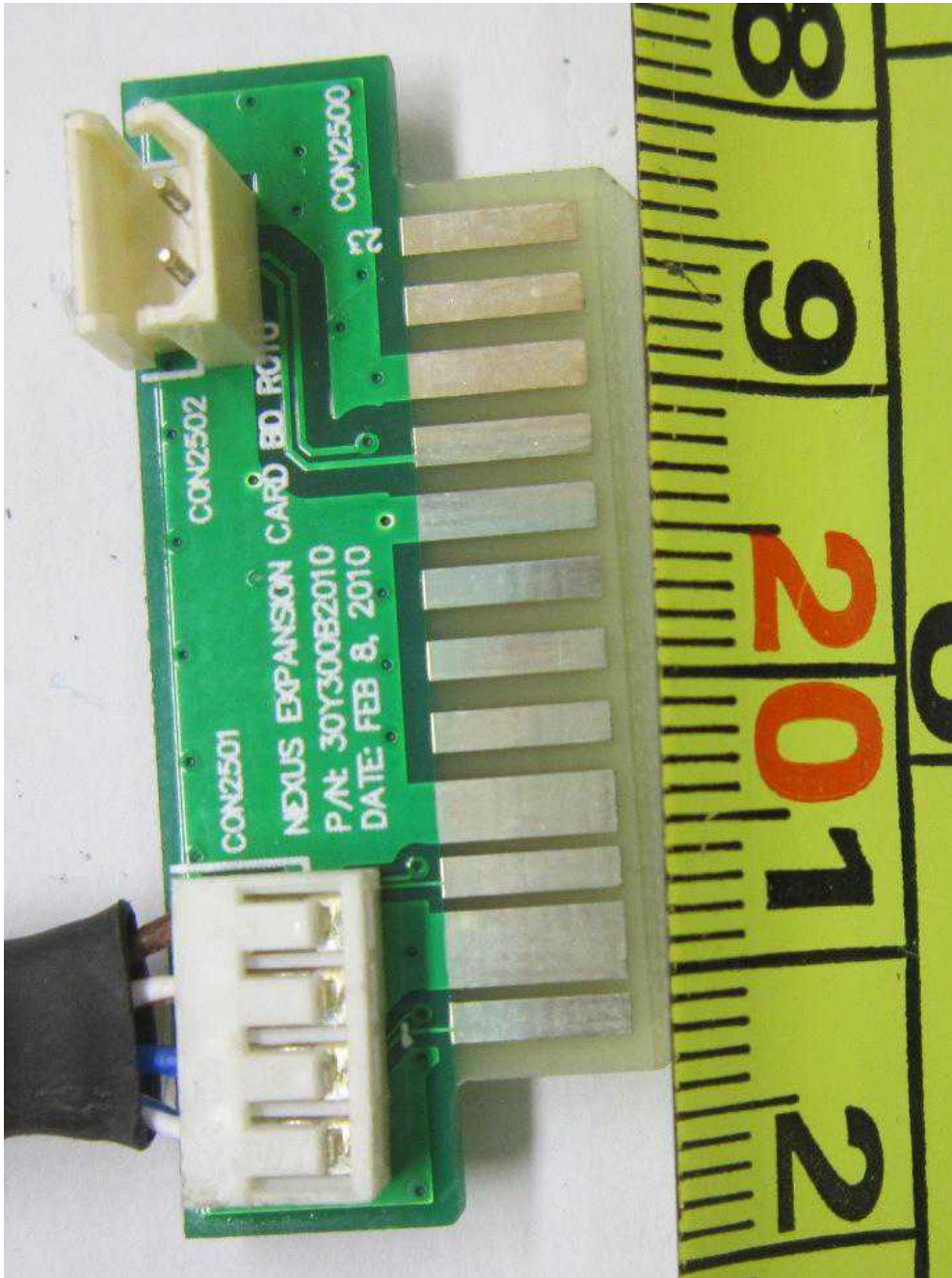
Adapter Board PCB Component Side
