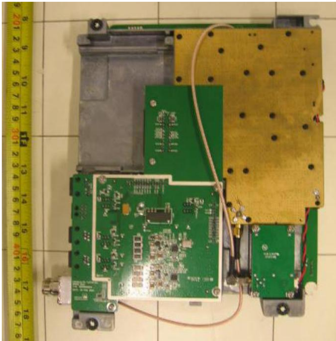
EUT PCB Trace Side
