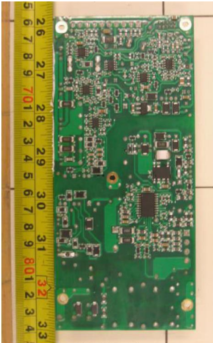
EUT PCB Trace Side
