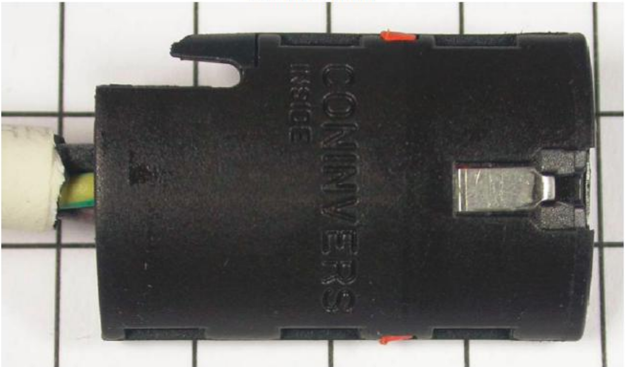
RolTop M10/17-915 AC cable connector
