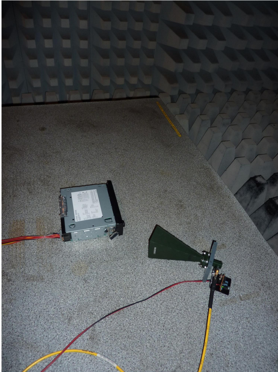
132962_03.JPG: Test setup fully anechoic chamber
