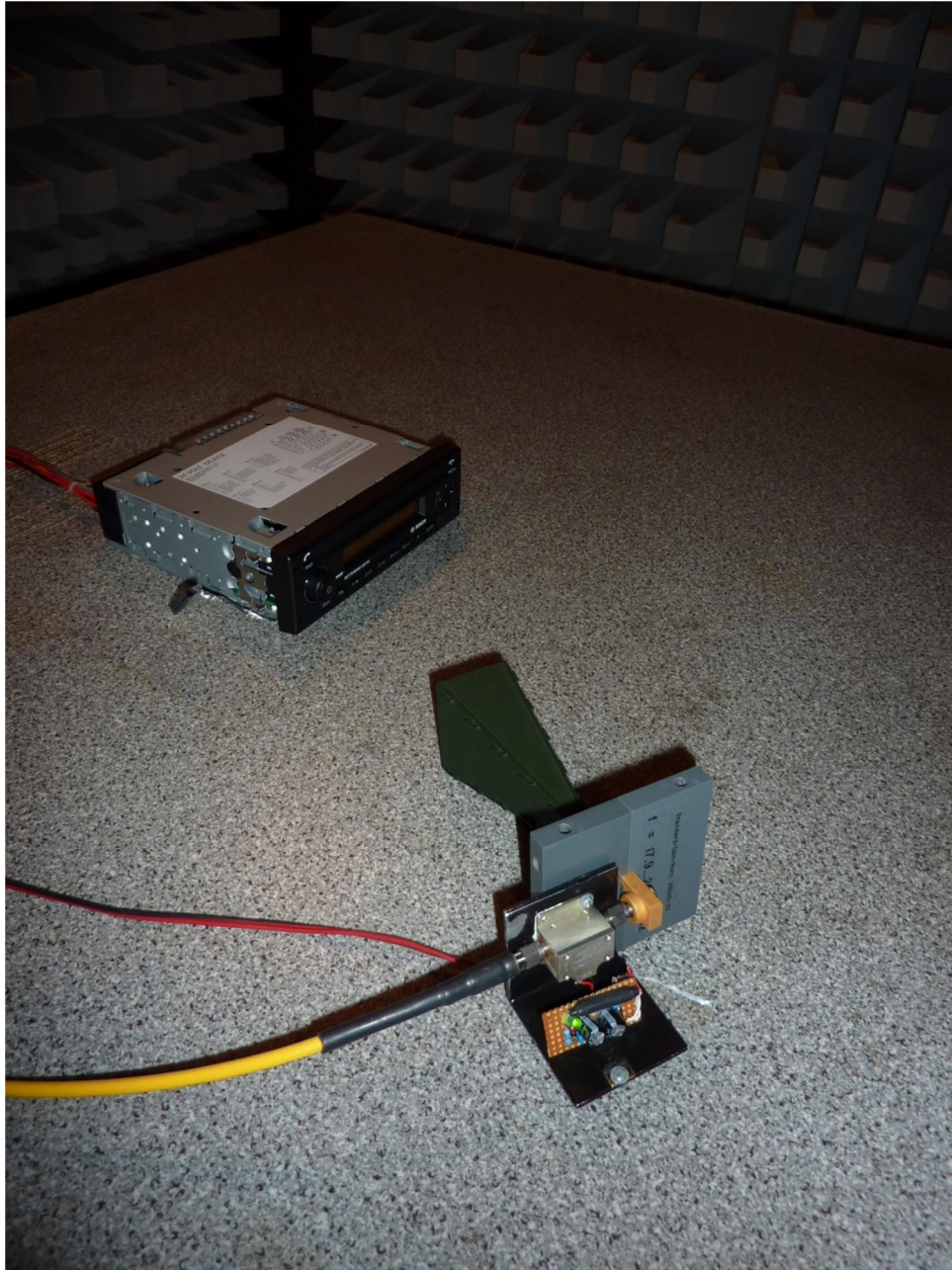
132962_04.JPG: Test setup fully anechoic chamber
