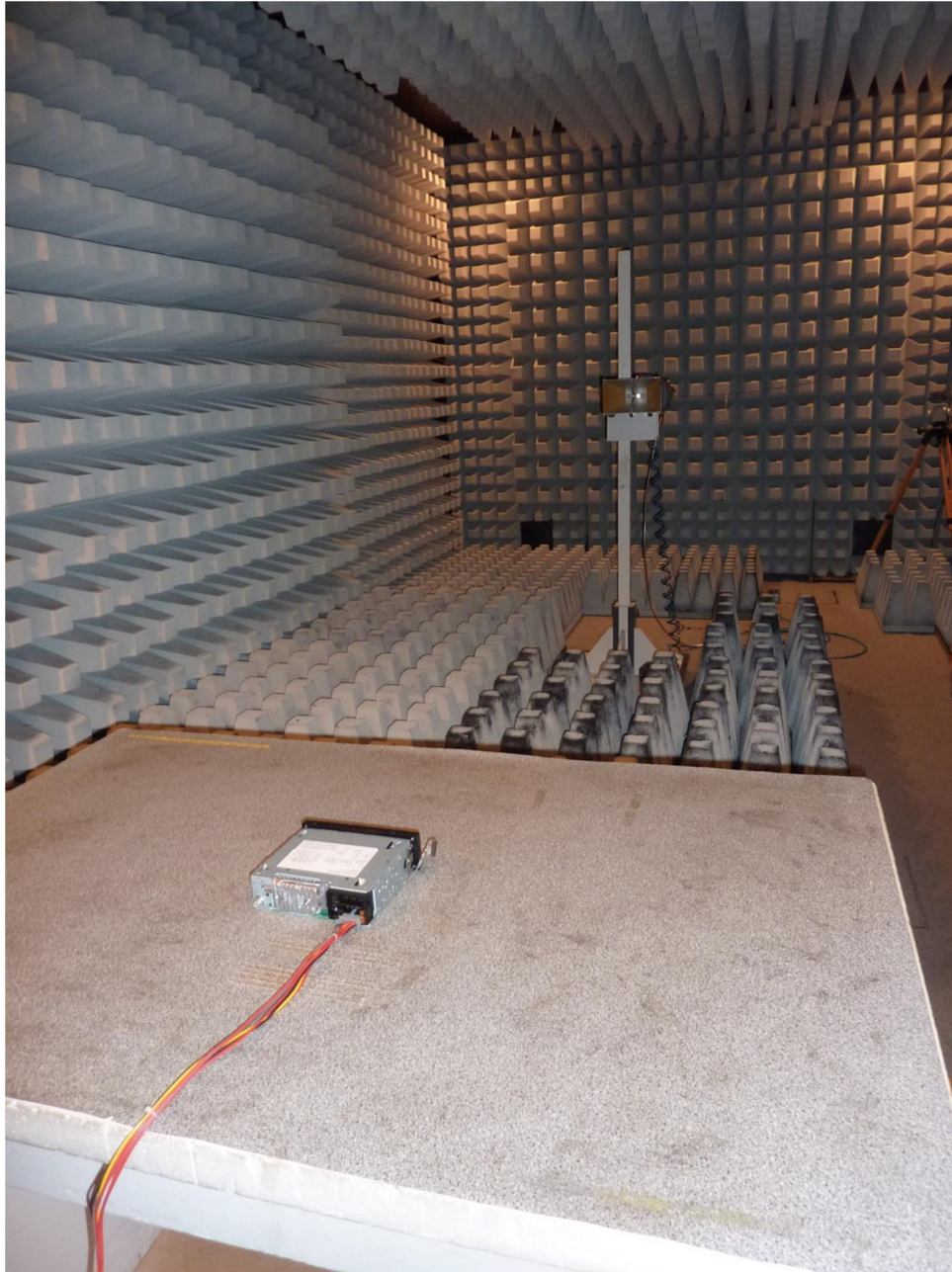
132962_01.JPG: Test setup fully anechoic chamber
