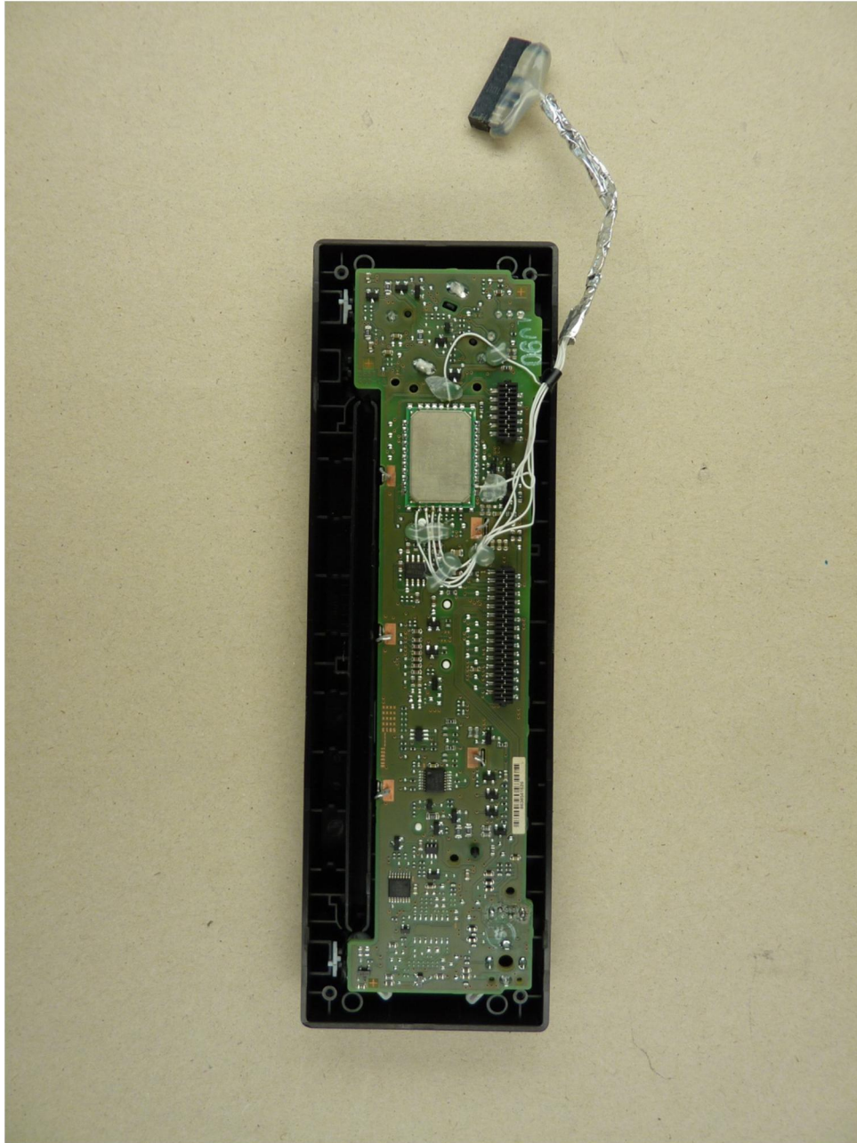
132962_14.JPG: Switch PCB, rear view
