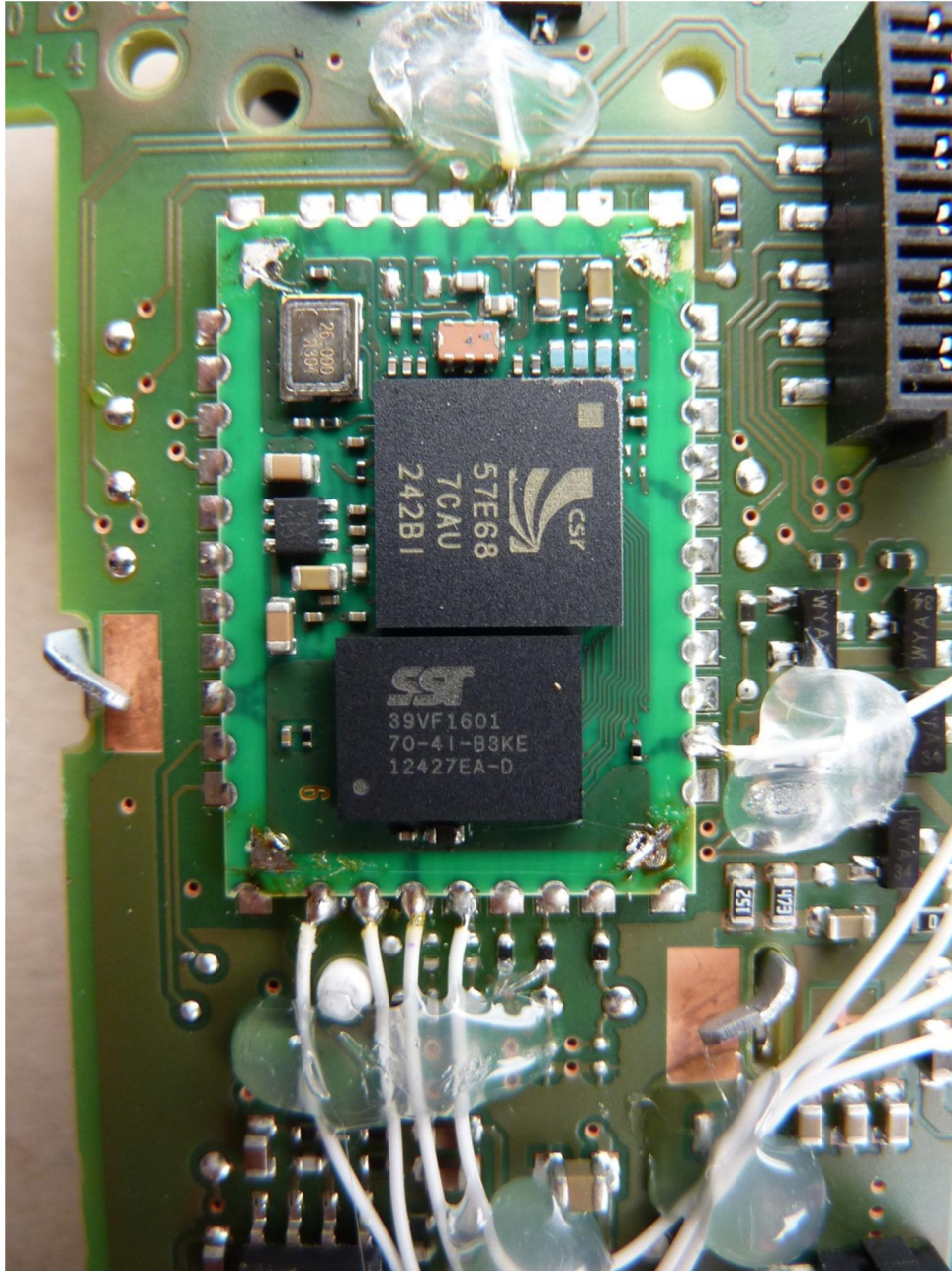
132962_18.JPG: Switch PCB, detail view to Bluetooth unit (unshielded)
