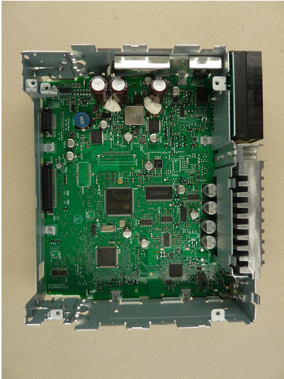
132962_11.JPG: Main PCB, top view
