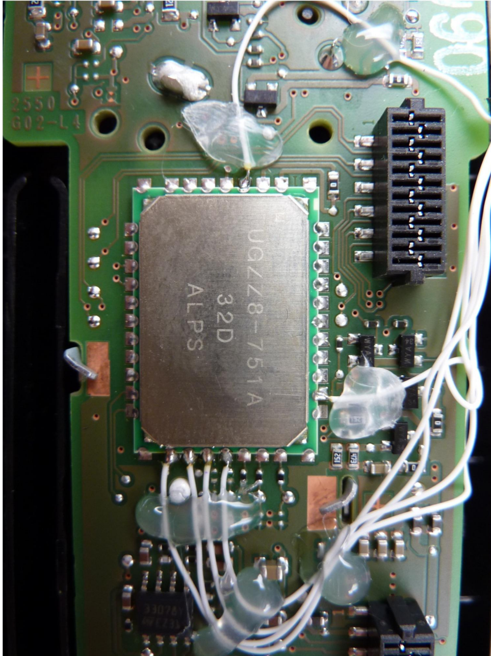
132962_15.JPG: Switch PCB, detail view to Bluetooth unit (shielded)
