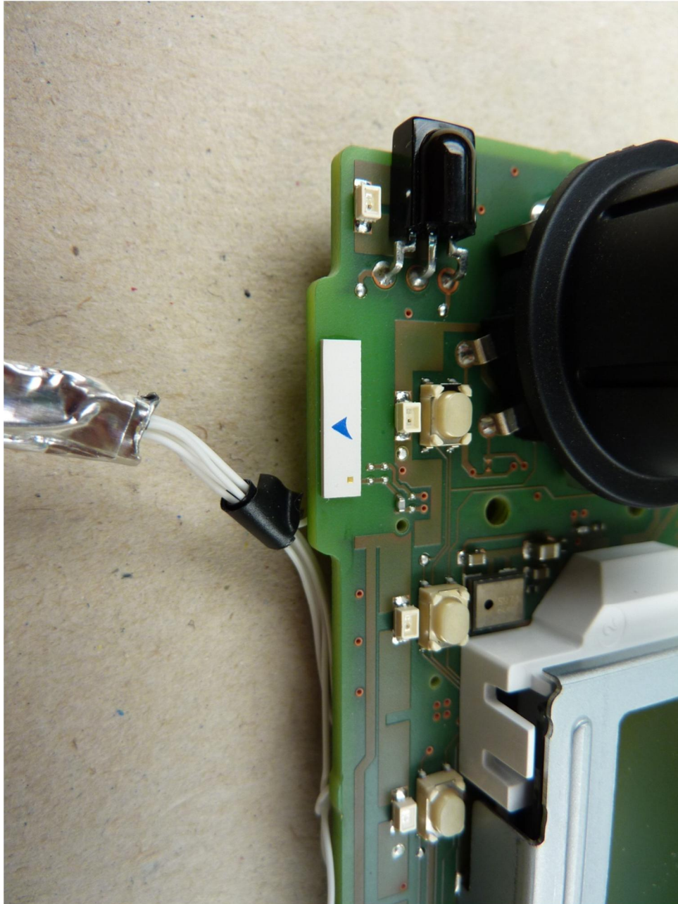
132962_17.JPG: Switch PCB, detail view to internal antenna
