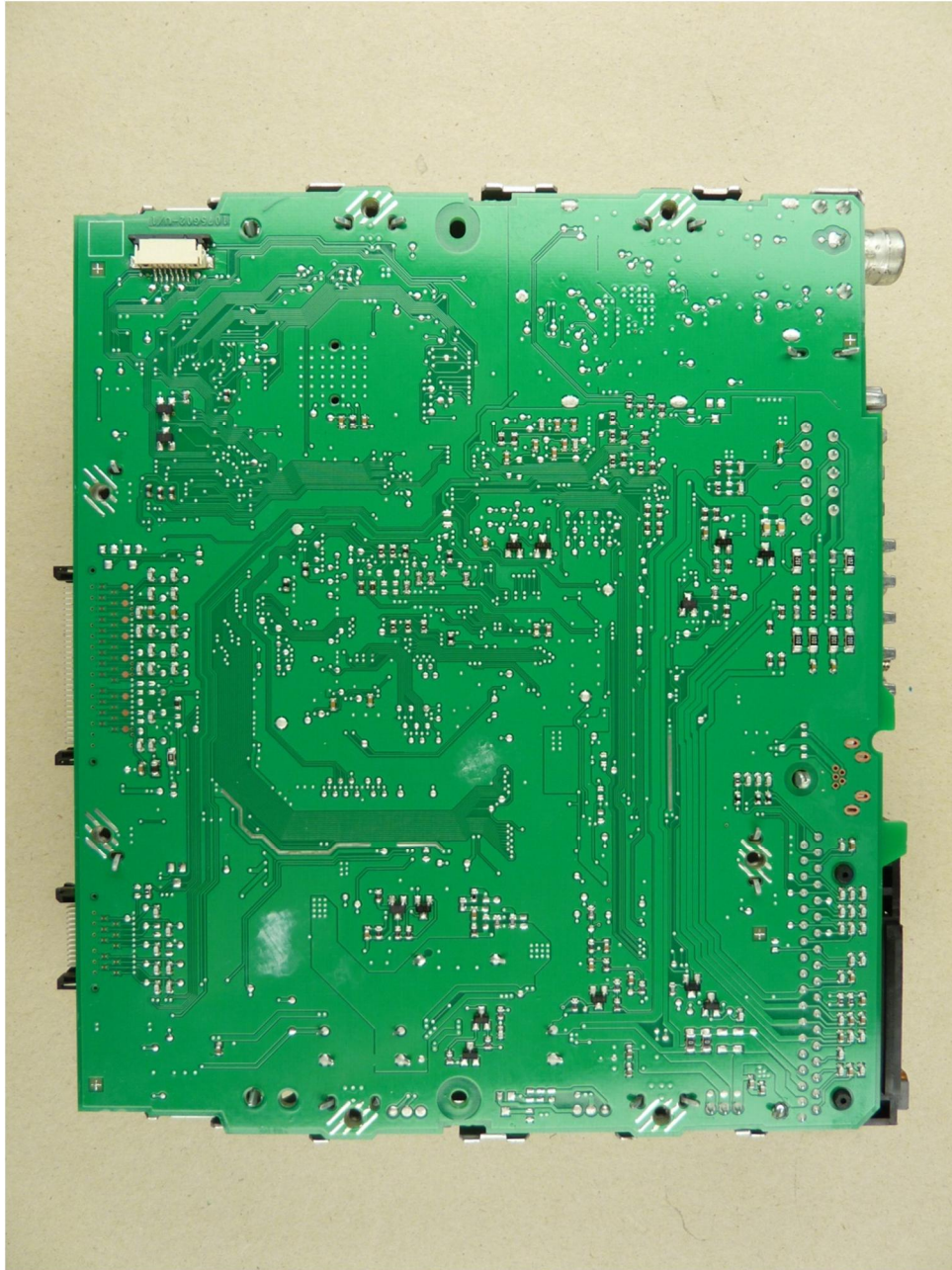
132962_12.JPG: Main PCB, bottom view
