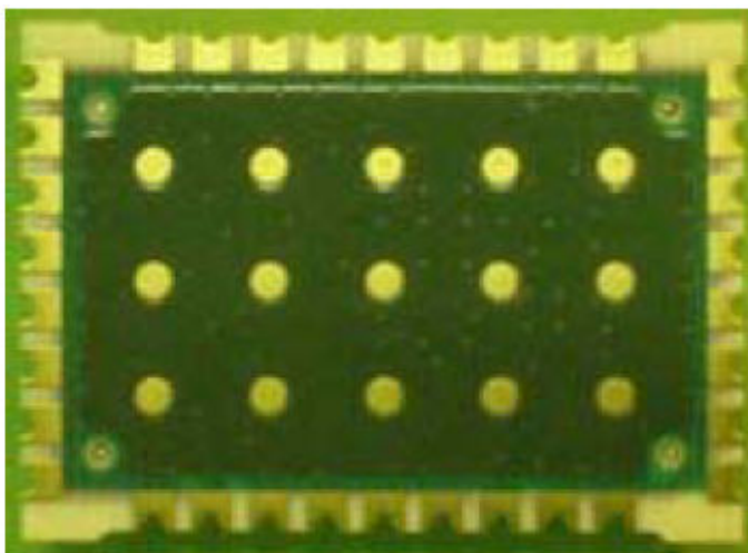
Top View – Internal (Shield casing removed)
