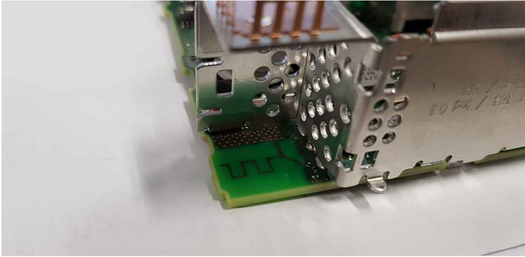
BT Antenna
