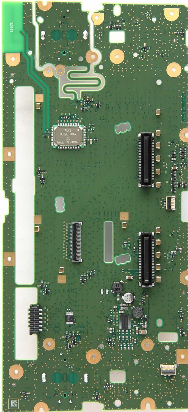
1.5. Photograph: Switchboard - bottom side view
