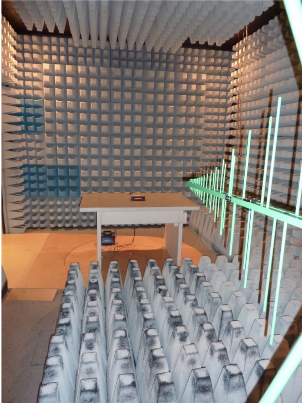
113093_08.JPG: Test setup fully anechoic chamber
