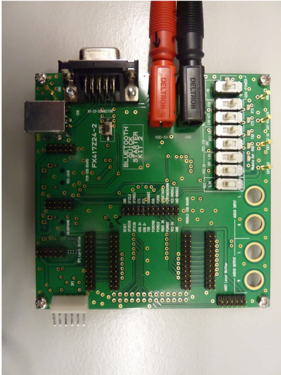
113093_EUT30.JPG: ALPS evaluation board, top view
