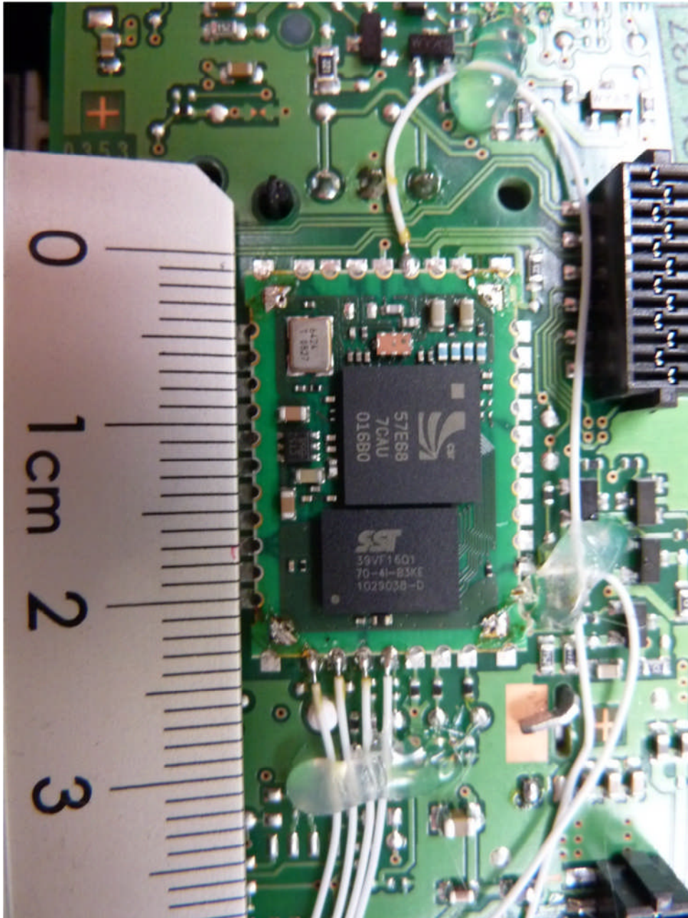
113093_EUT33.JPG: Switch PCB, detail view to Bluetooth unit (unshielded)
