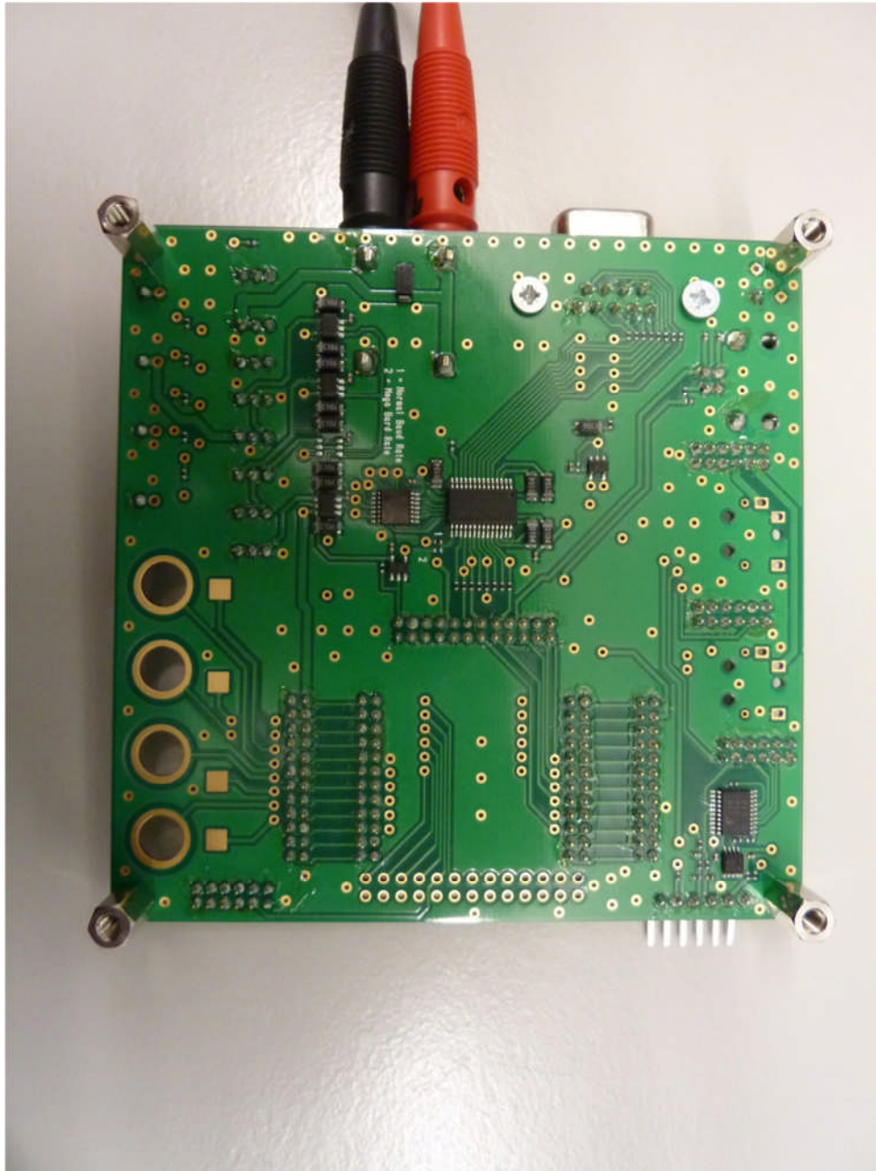
113093_EUT31.JPG: ALPS evaluation board, bottom view
