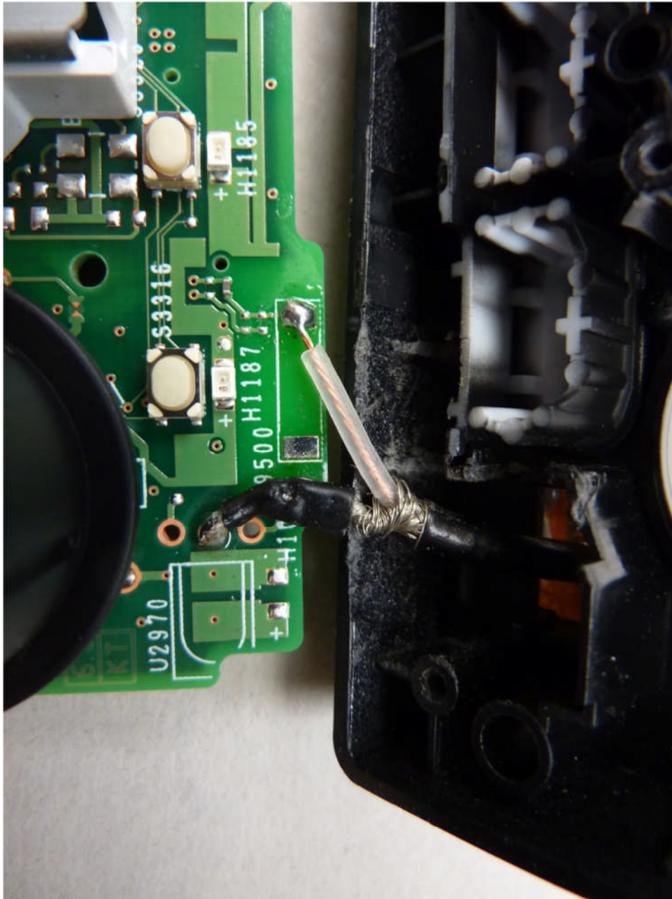
113093_EUT27.JPG: Switch PCB, detail view to temporary antenna connector
