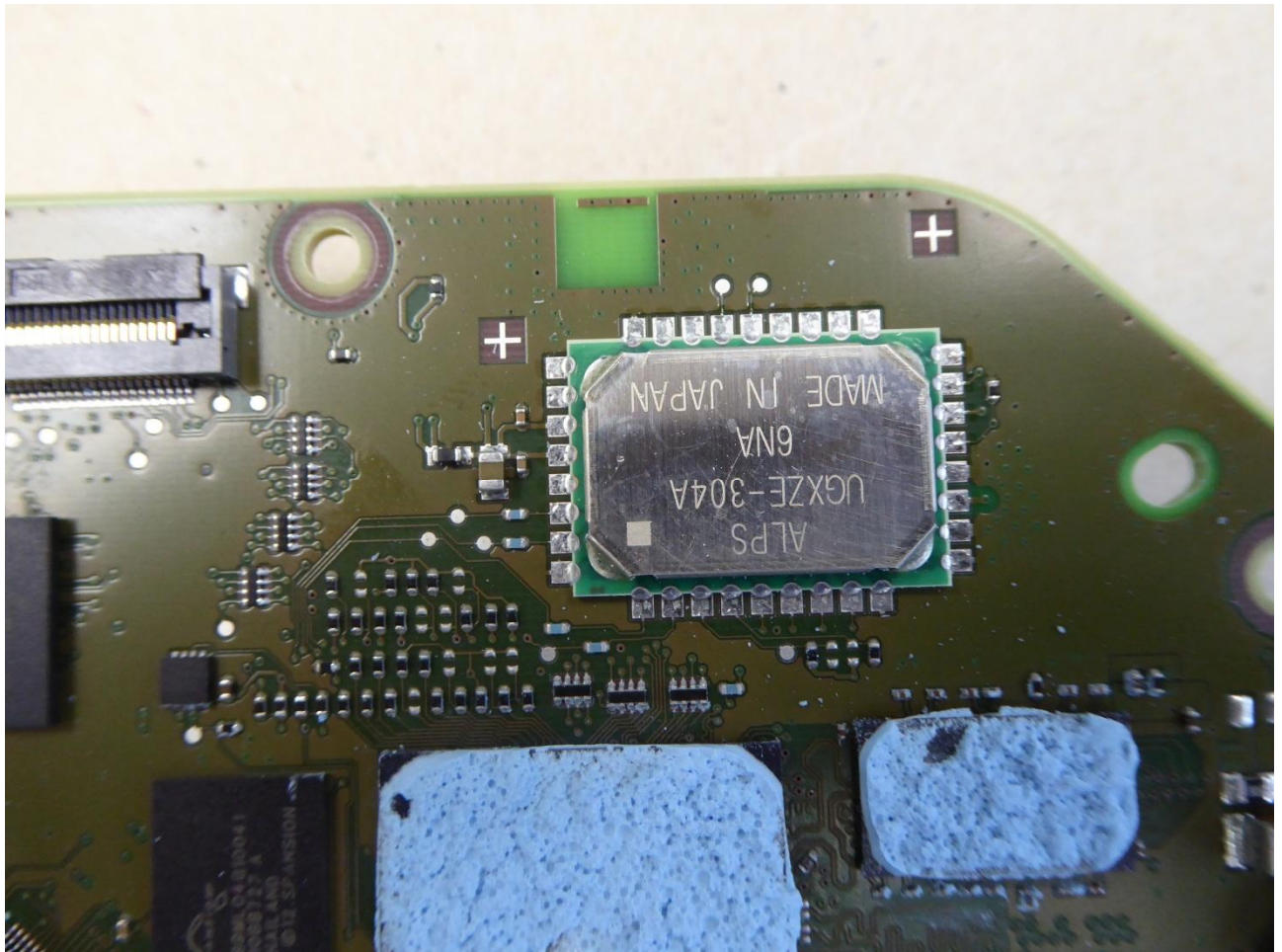
162097_21.jpg: EUT #005 – UGXZEX304A module – close-up
