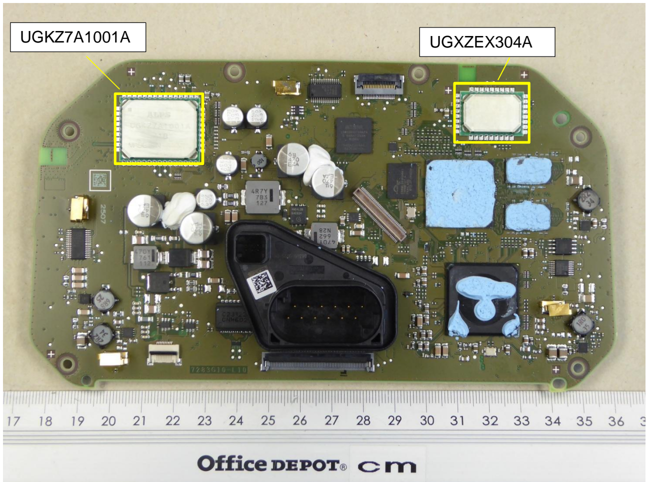
162097_15.jpg: EUT #005 – Main PCB top view
