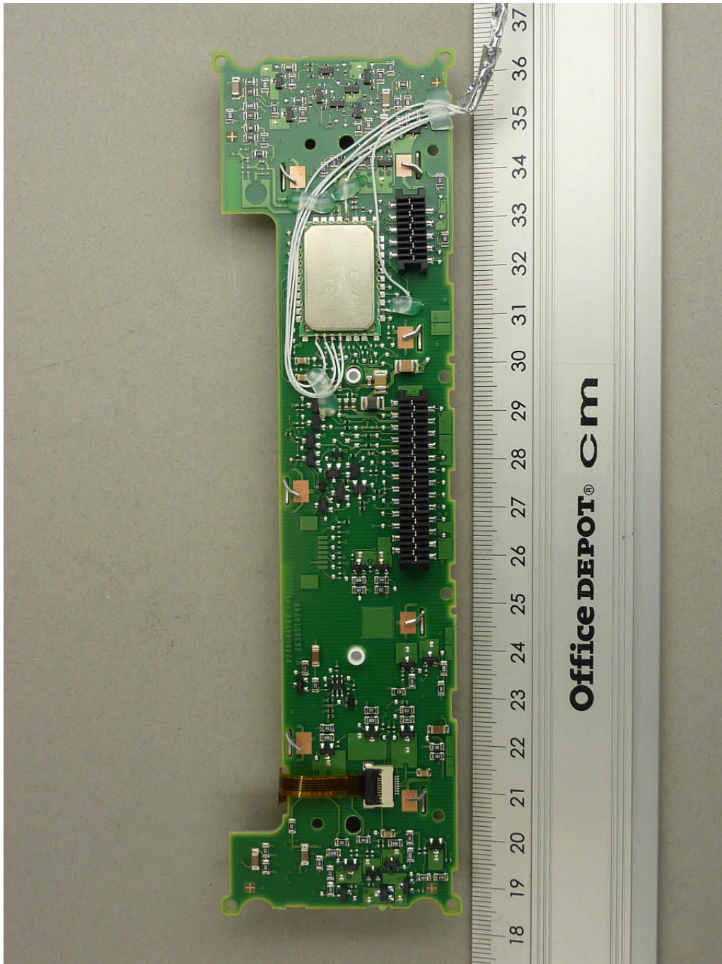
110734_d.jpg Switch PCB, rear view
