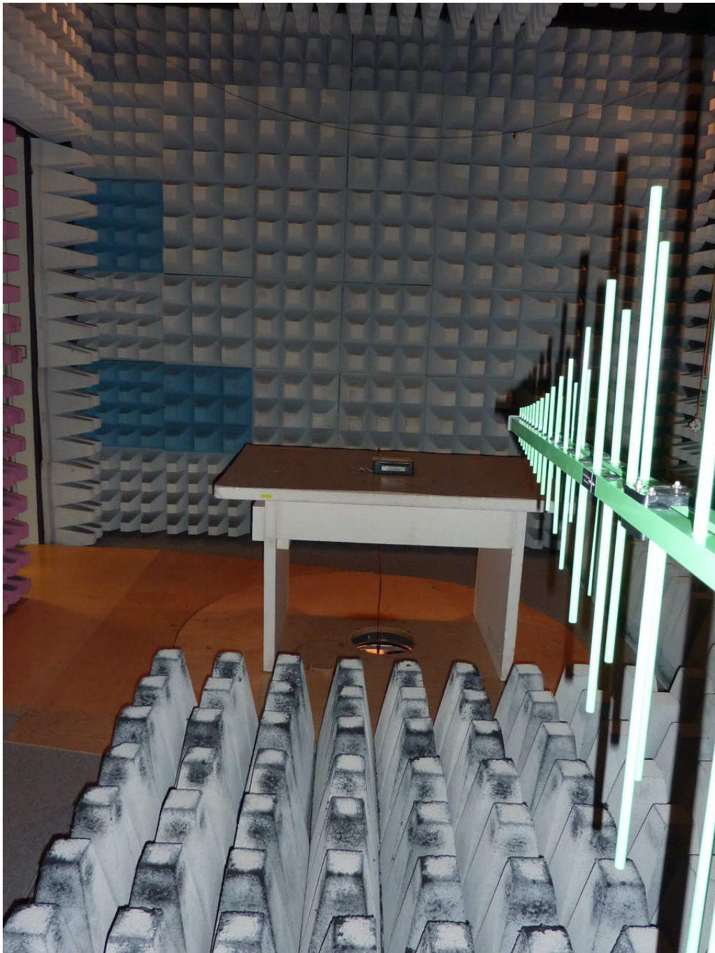
110734_9.jpg Test set-up fully anechoic chamber
