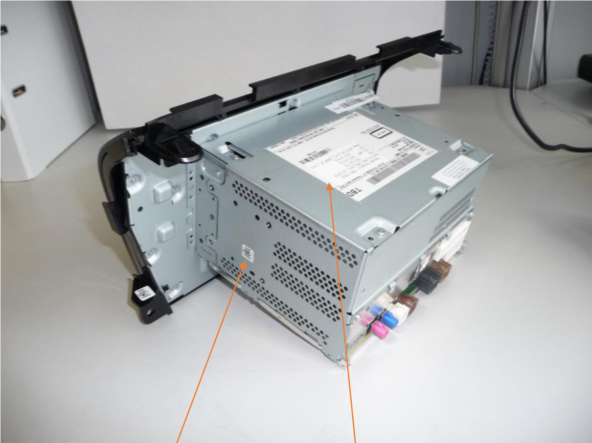
AIVIP42M0 with Draft labels: 1) Bosch label with Dot matrix code; 2) Customer label for displaying all necessary certification information (e.g. for FCC).
