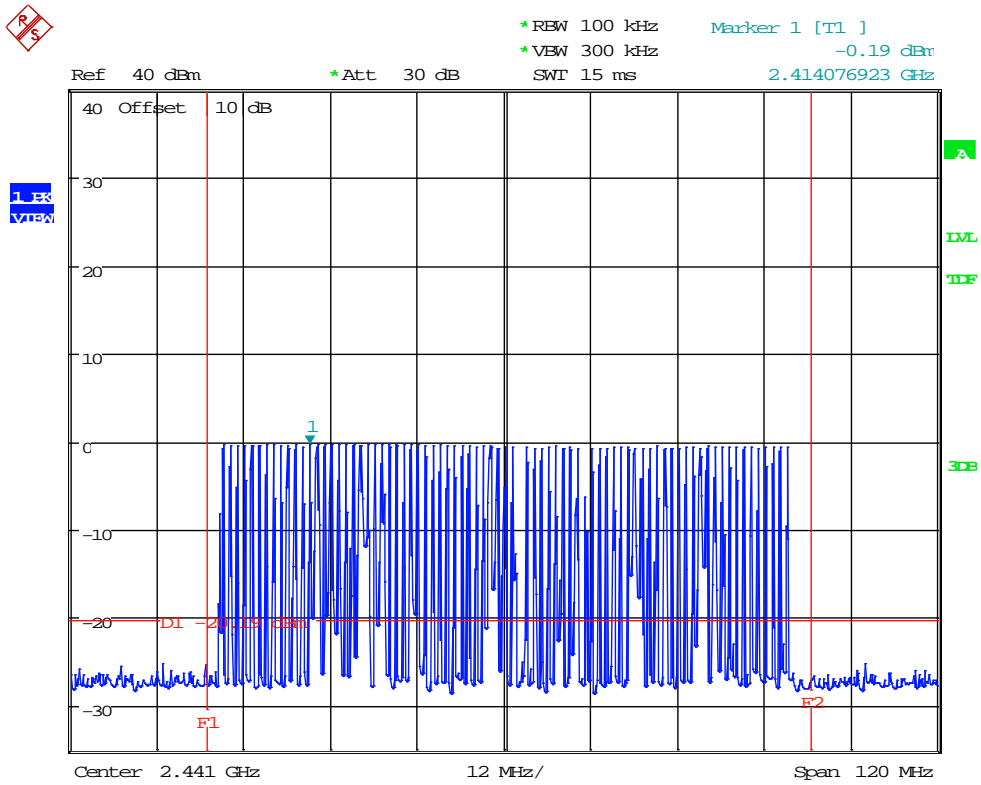
Plot 26: 20dBc Ref | 2-DH5 | pi/4 QPSK | Ch 39 (2442 MHz)
