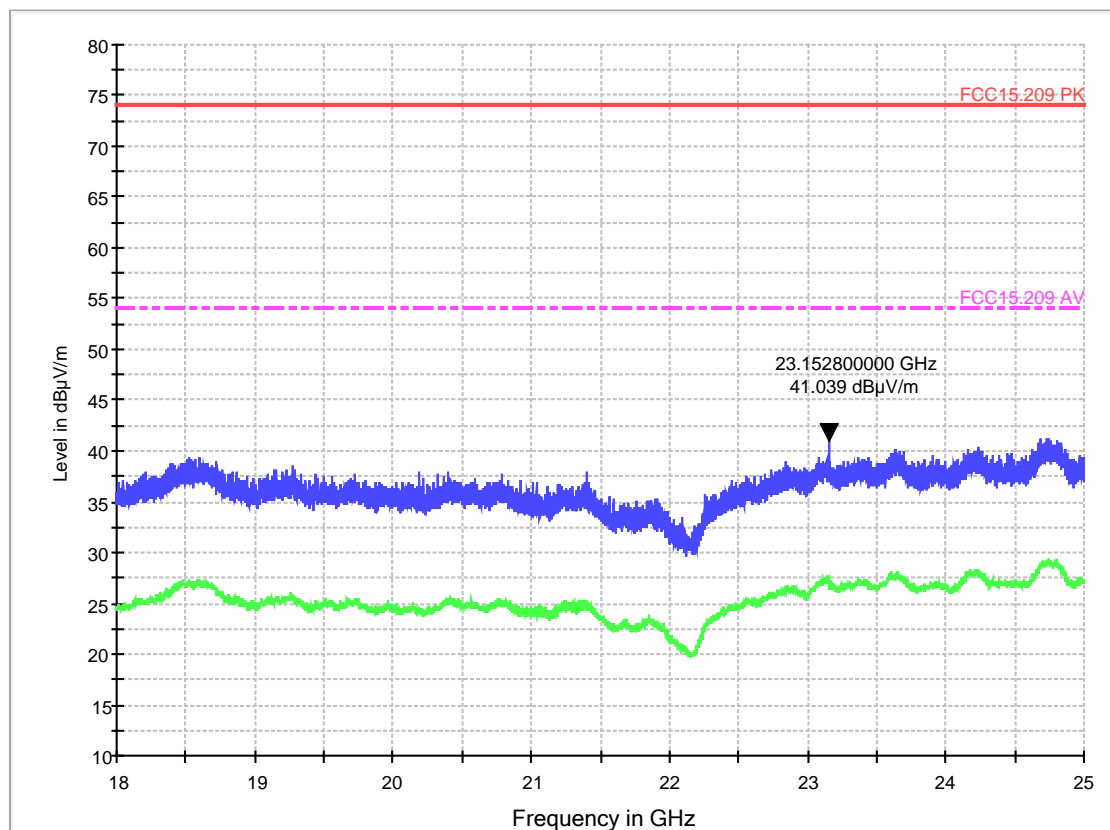
EMI Scan_18_25GHz_Pre
