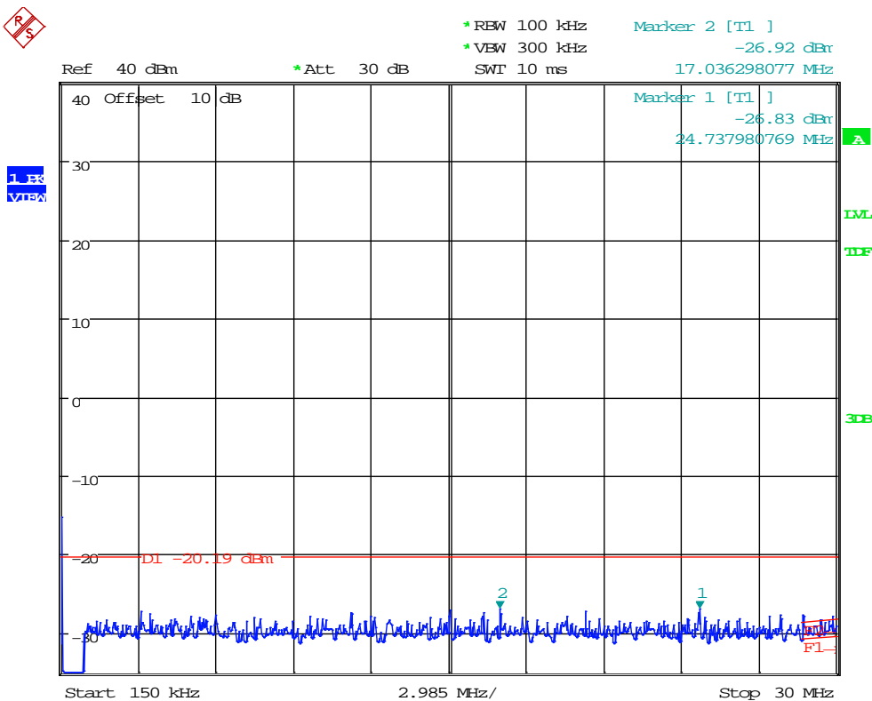
Plot 27: 20dBc | 0.15-30MHz | 2-DH5 | pi/4 QPSK | Ch 39 (2442 MHz)
