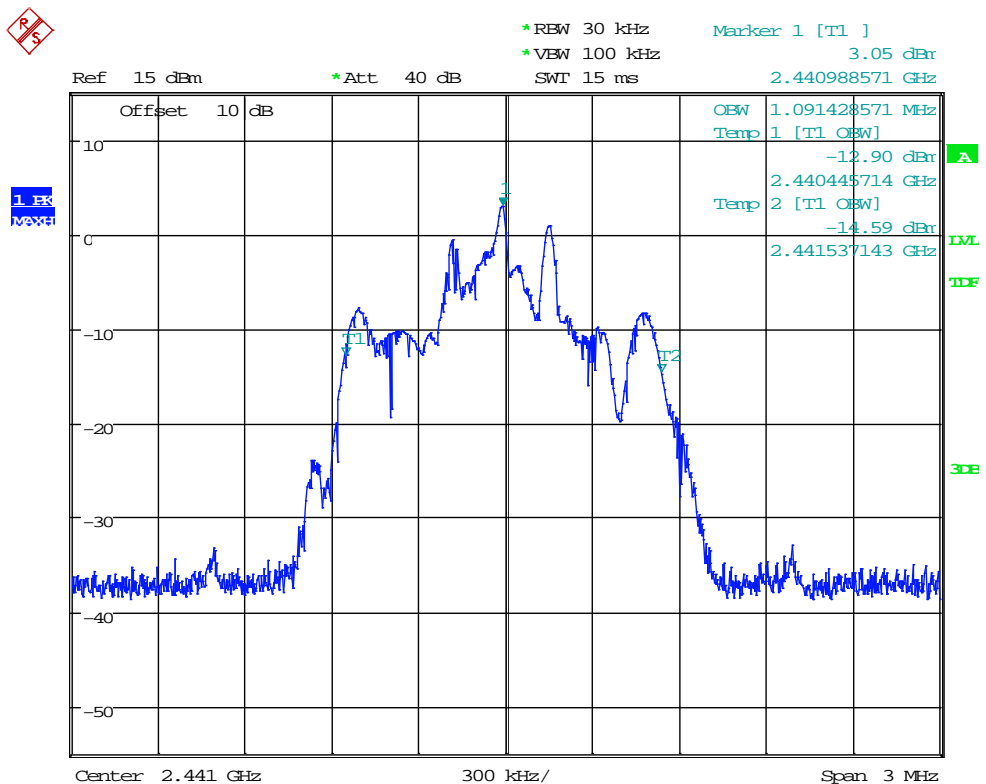
Plot 8: 99%BW_BT_3-DH3_ch39
