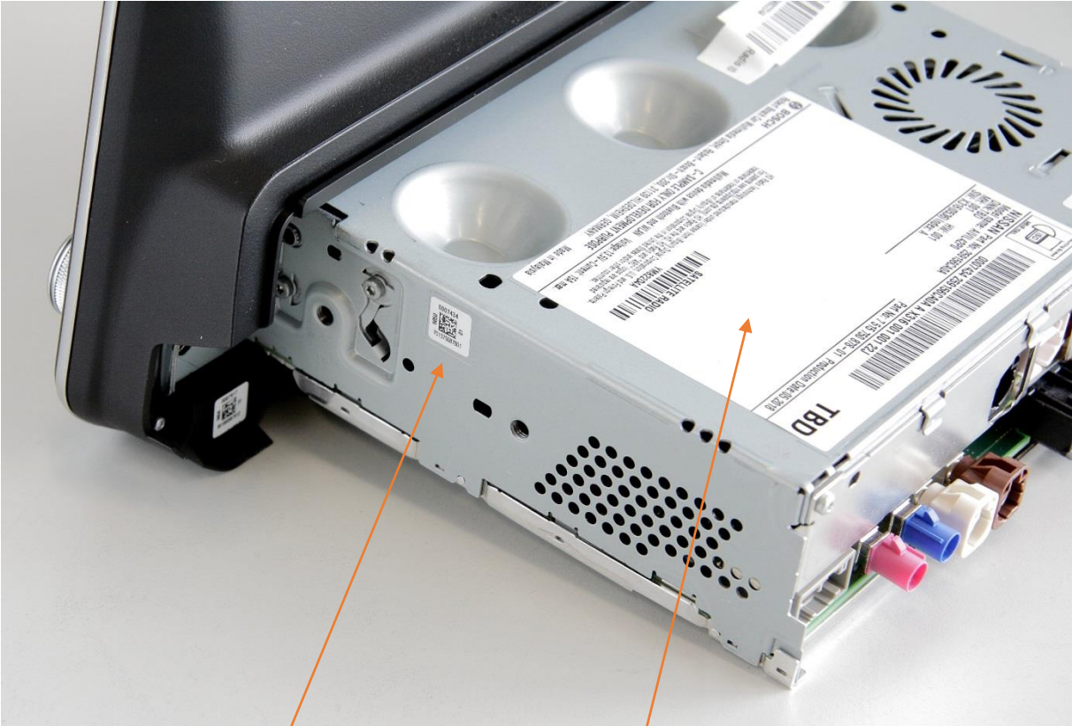
AIVIL43P0 with Draft labels: 1) Bosch label with Dot matrix code; 2) Customer label for displaying all necessary certification information (e.g. for FCC). Both label positions are described in the document 7500750828-A.pdf
